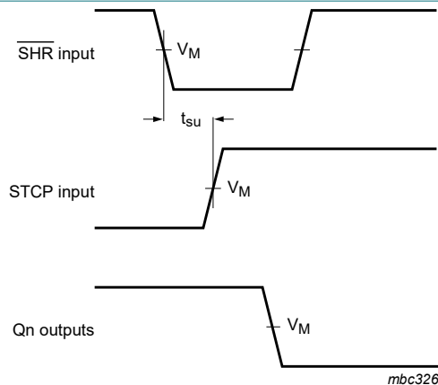
Fig. 10. The shift reset ( \overline{\text{SHR}} ) to storage clock (STCP) set-up times
