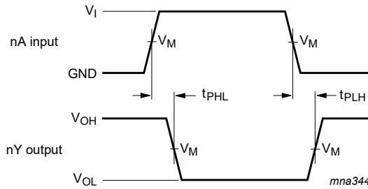
Fig. 9. The data input (nA) to output (nY) propagation delays
