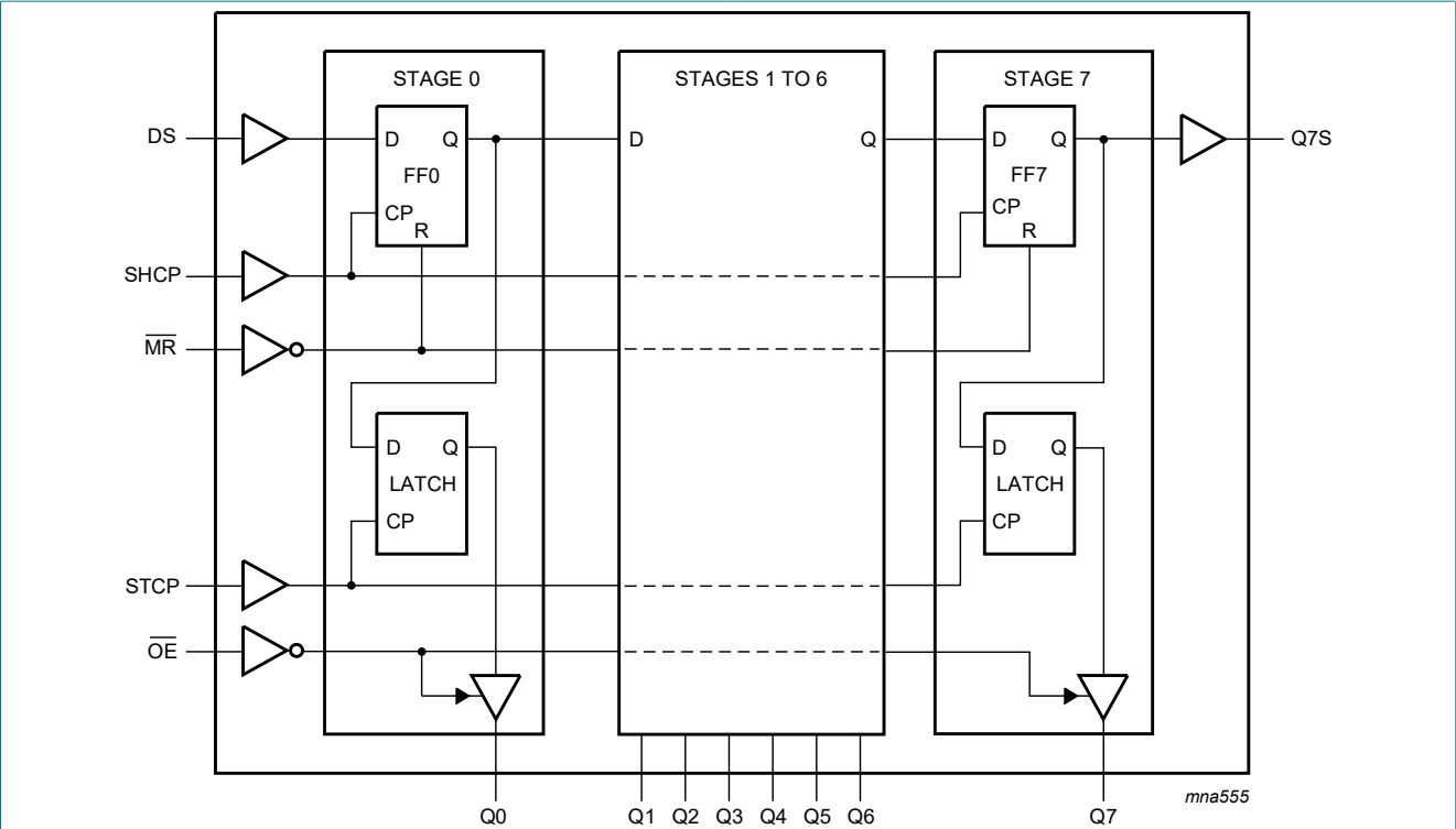
Fig. 4. Logic diagram
