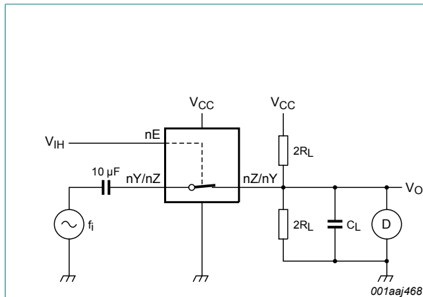
Fig. 11. Test circuit for measuring total harmonic distortion
