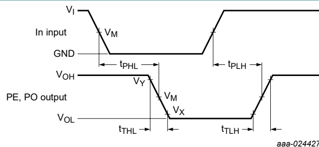
Fig. 5. Input (In) to output (PE, PO) propagation delays and output transition times
