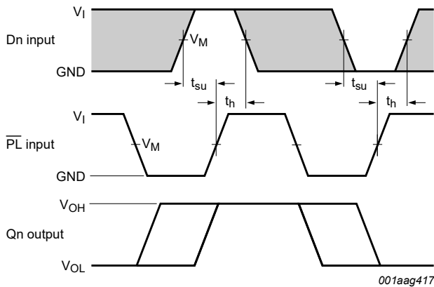
Measurement points are given in Table 10. V_{OL} and V_{OH} are typical voltage output levels that occur with the output load. The shaded areas indicate when the input is permitted to change for predictable output performance.
