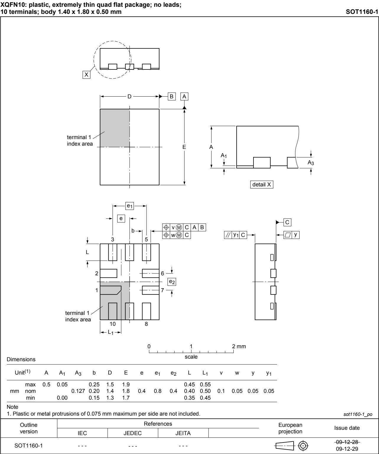
Fig. 11. Package outline SOT1160-1 (XQFN10)
