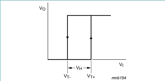
Fig. 8. Transfer characteristic
