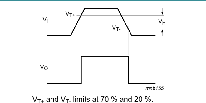
Fig. 9. Definition of V_{T+} , V_{T-} and V_H
