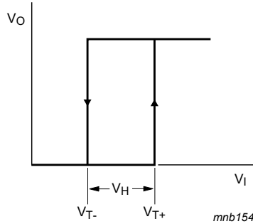
Fig. 7. Transfer characteristic
