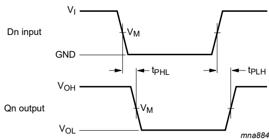
Fig. 8. Input Dn to output Qn propagation delay times
