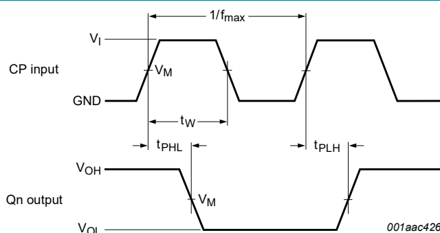
Fig. 7. Clock pulse width, maximum frequency and input to output propagation delays
