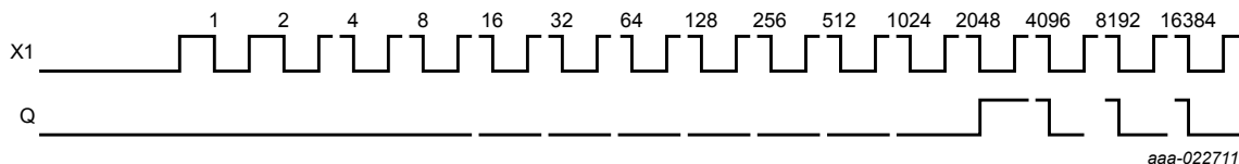
Figure 4. Timing diagram
