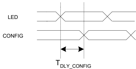
Figure 31: LED to CONFIG Timing
