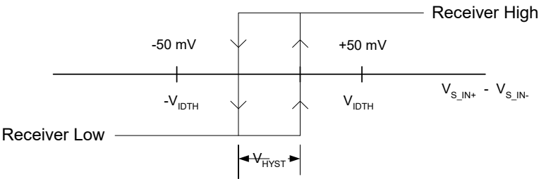
Figure 27: Input Differential Hysteresis
