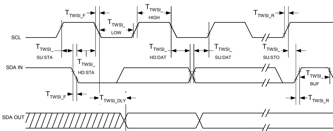
Figure 34: TWSI Master Timing
