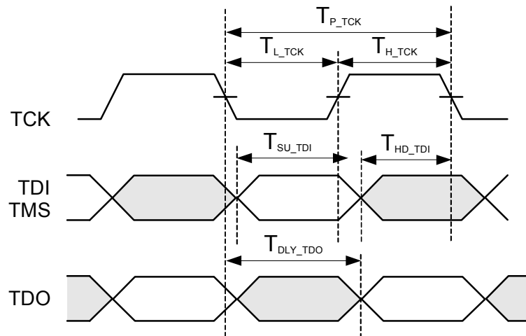
Figure 33: JTAG Timing
