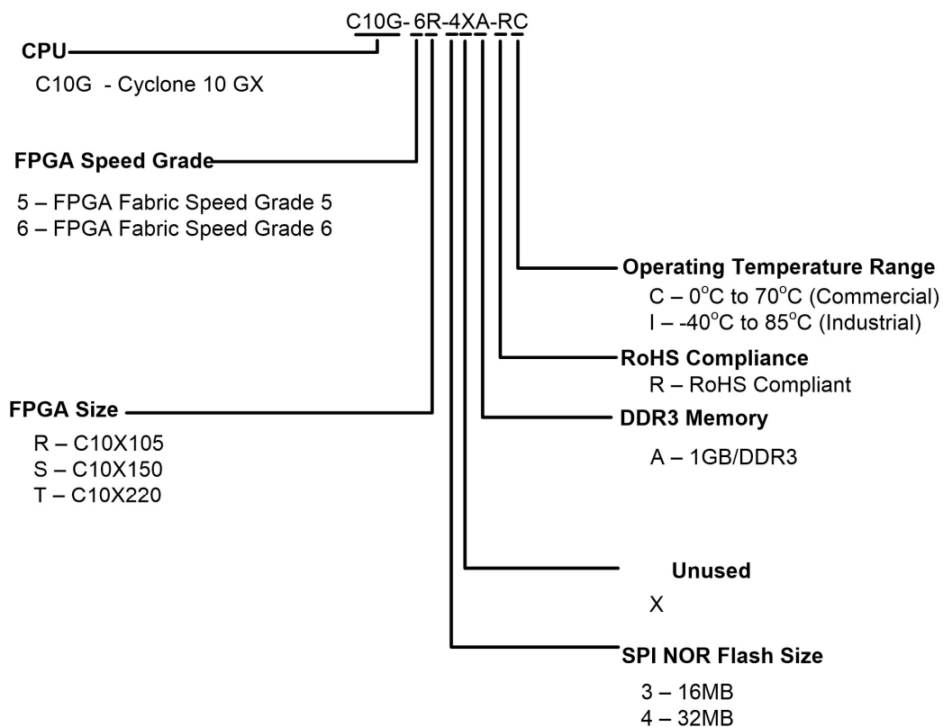
Figure 3 MitySOM-C10G Model Number Decoder
