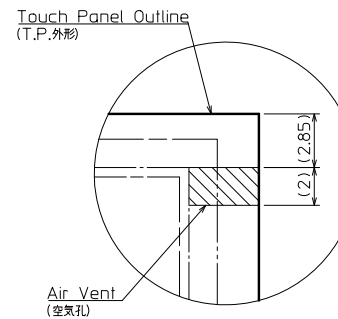
DETAIL B (5:1)
