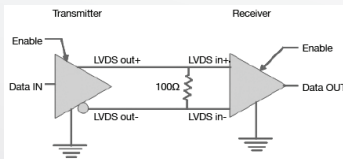
LVDS Interface
