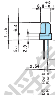
推奨取付寸法 Recommended mounting dimensions
