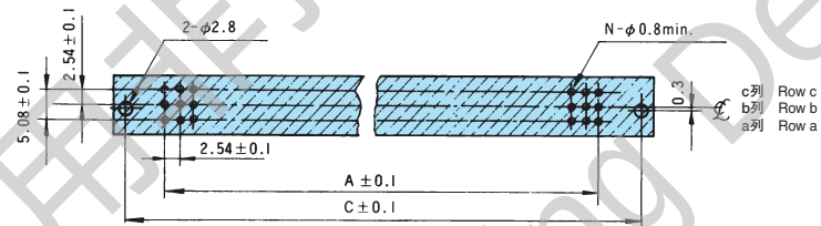
推奨取付寸法 Recommended mounting dimensions
