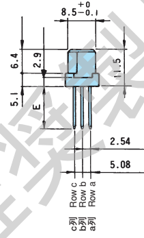
推奨取付寸法 Recommended mounting dimensions
