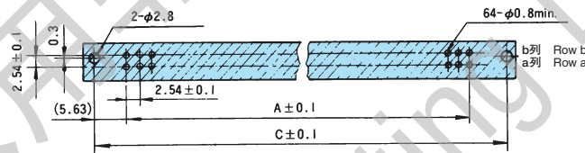
推奨取付寸法 Recommended mounting dimensions
