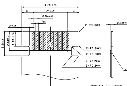
推奨FPC/FFC寸法 RECOMMENDED FPC/FFC
