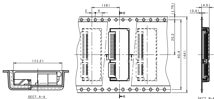
SECT. B-B
