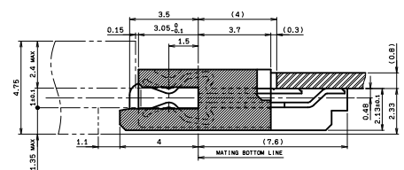
MATING CONDITION
