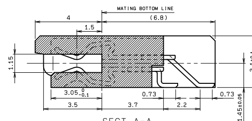
SECT. A-A
