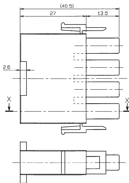
SECT. X-X
