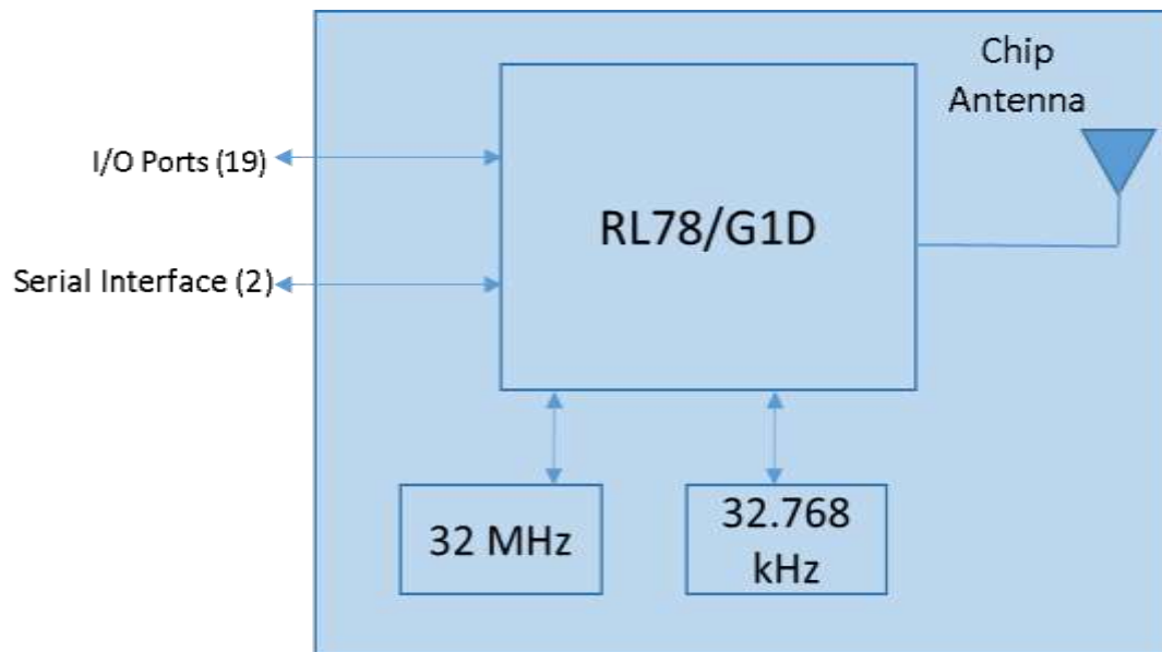
Figure 1 ISM78G1D-L31 Block Diagram
