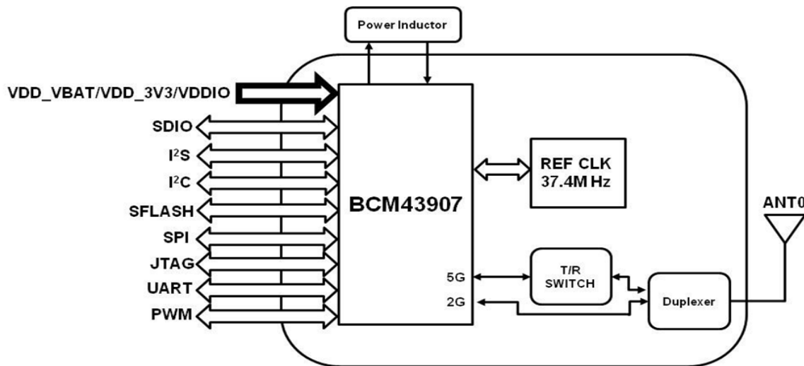
ISM43907-L170-EVB Diagram
