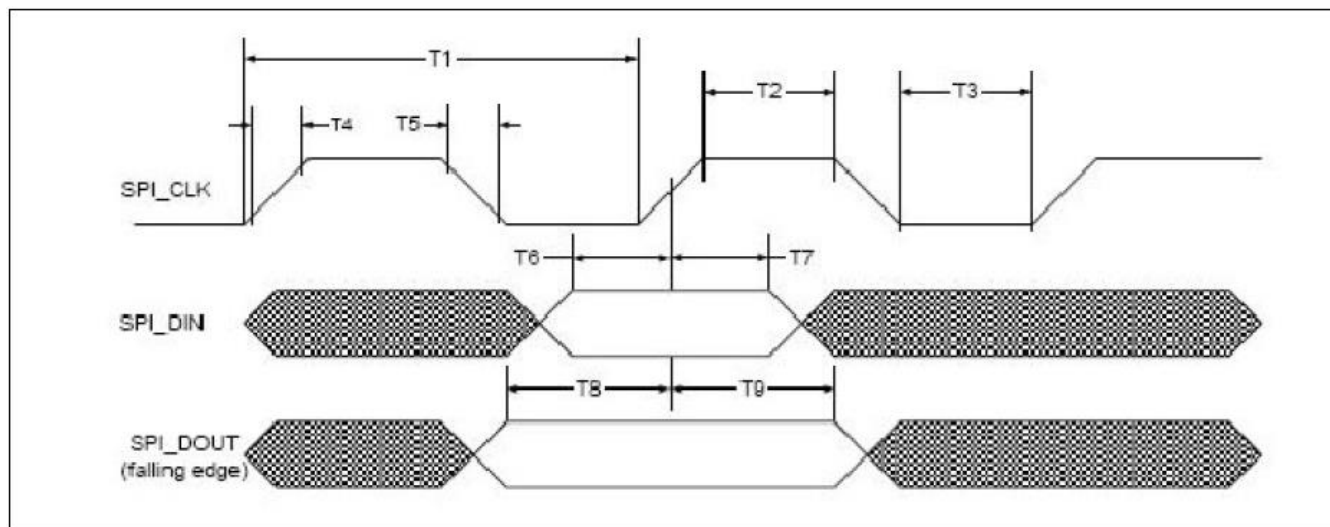
gSPI Timing
