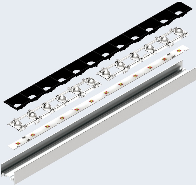
Exploded view with aluminium profile
