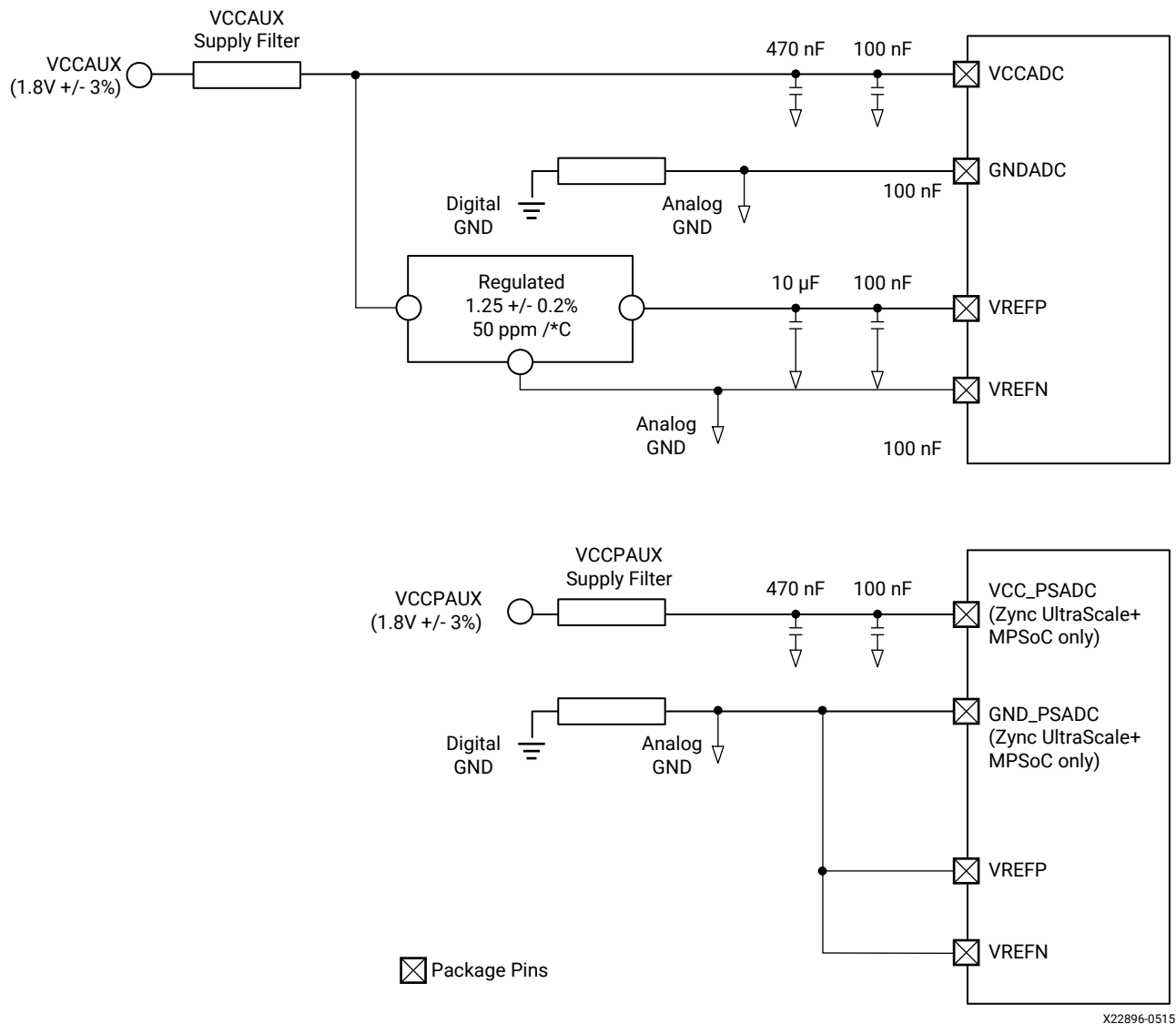
Figure 10: PL and PS SYSMON Power Connections
