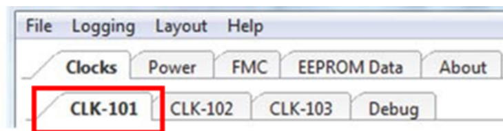
Figure 26: CLK-101 Tab
