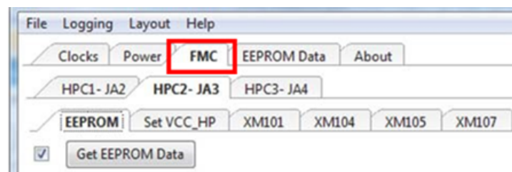
Figure 42: FMC Tab
