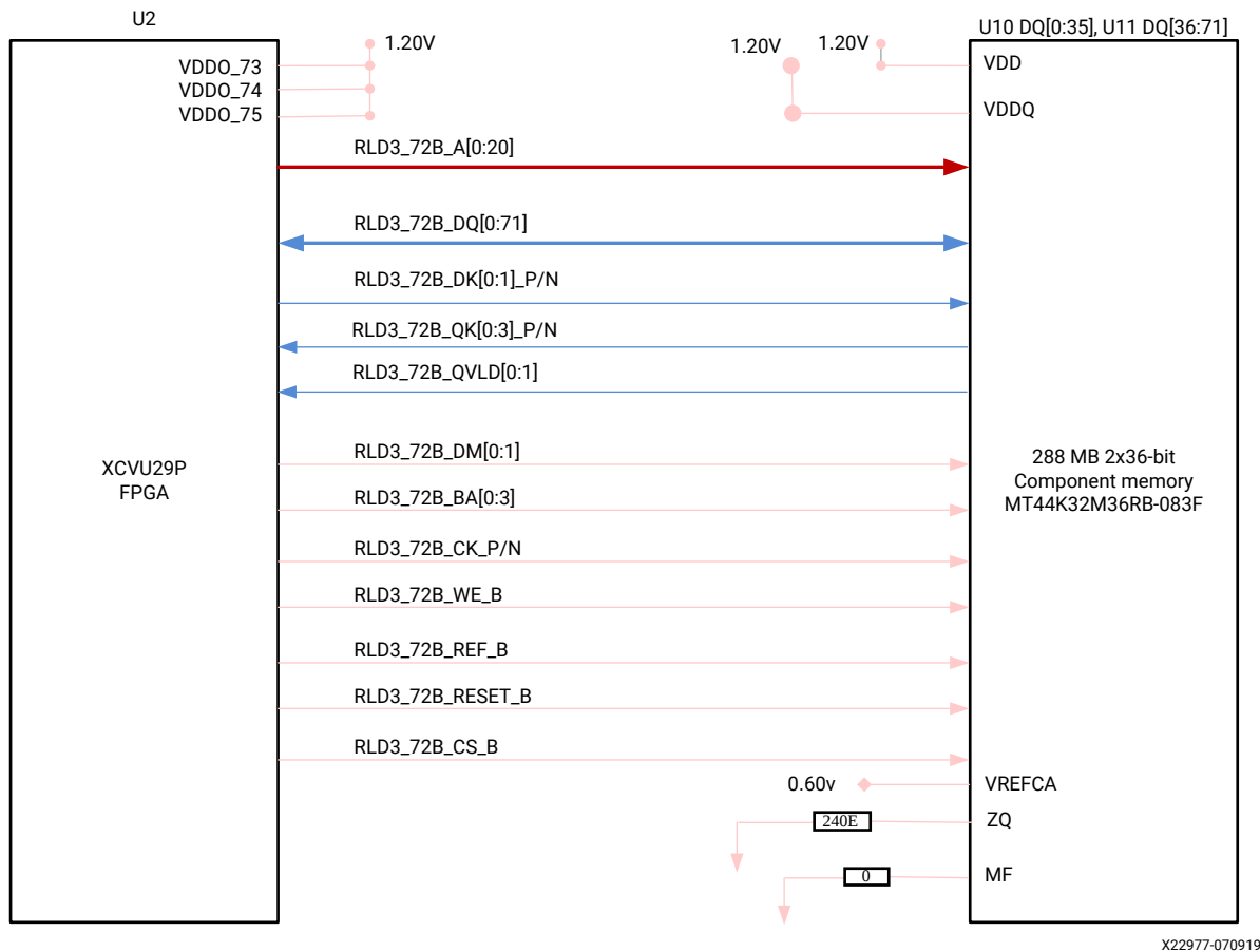
Figure 5: RLD3 Memory Interface
