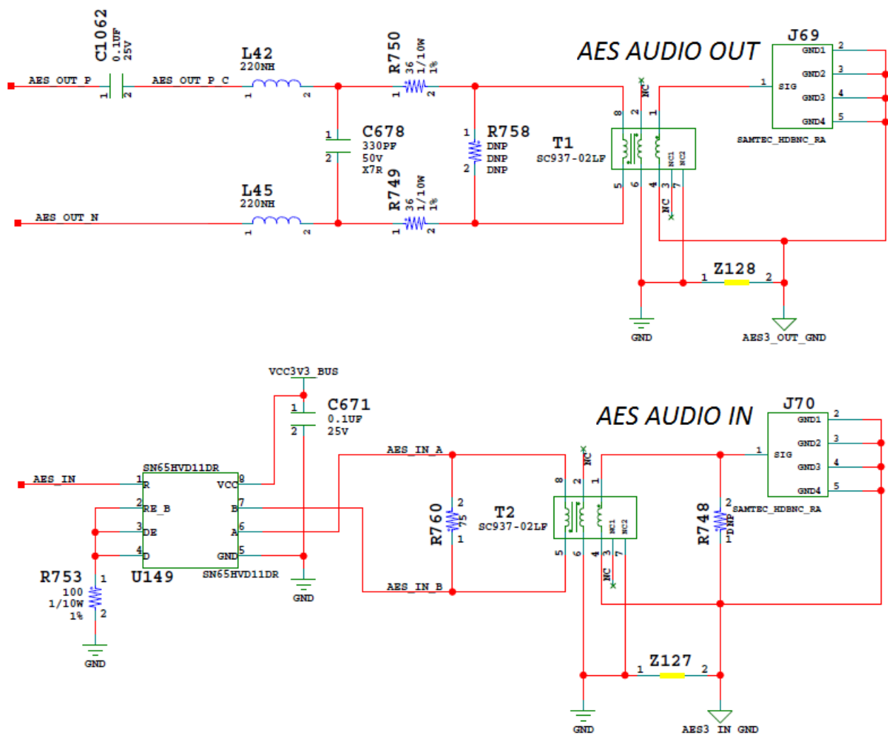
Figure 3-28: AES Audio
