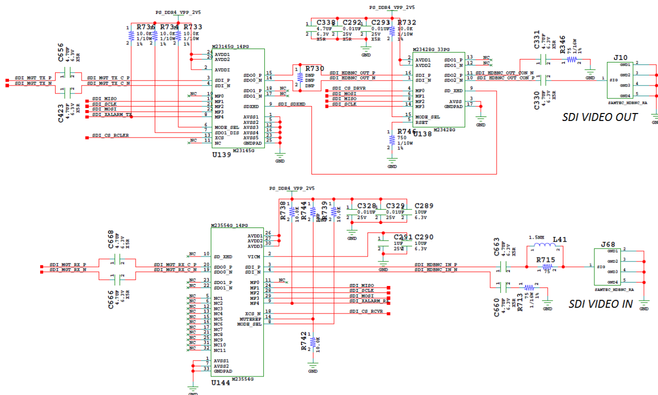
Figure 3-27: SDI Video
