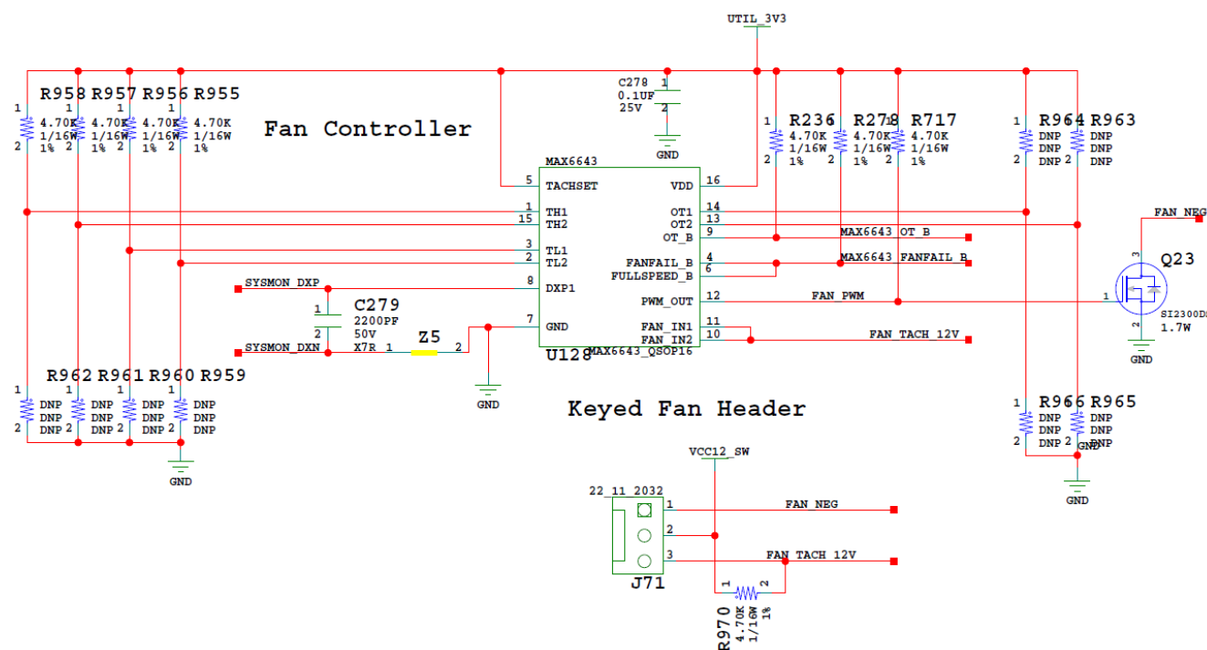
Figure 3-43: ZCU106 12V Fan Controller
