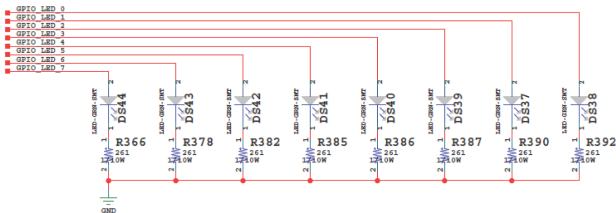
Figure 3-34: GPIO LEDs
