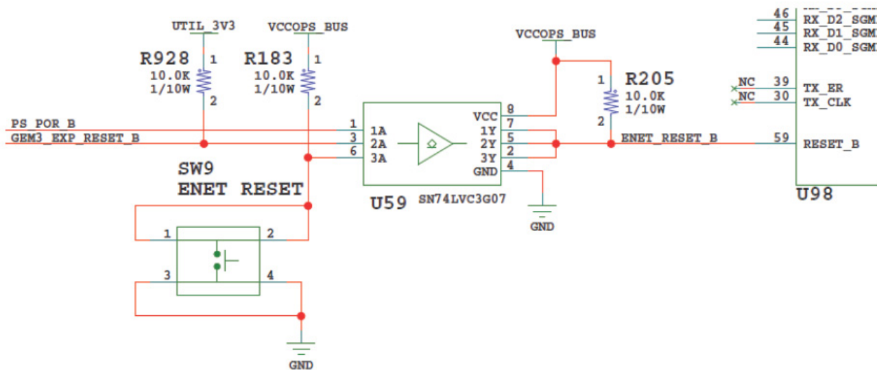
Figure 3-13: Ethernet PHY Reset Circuit
