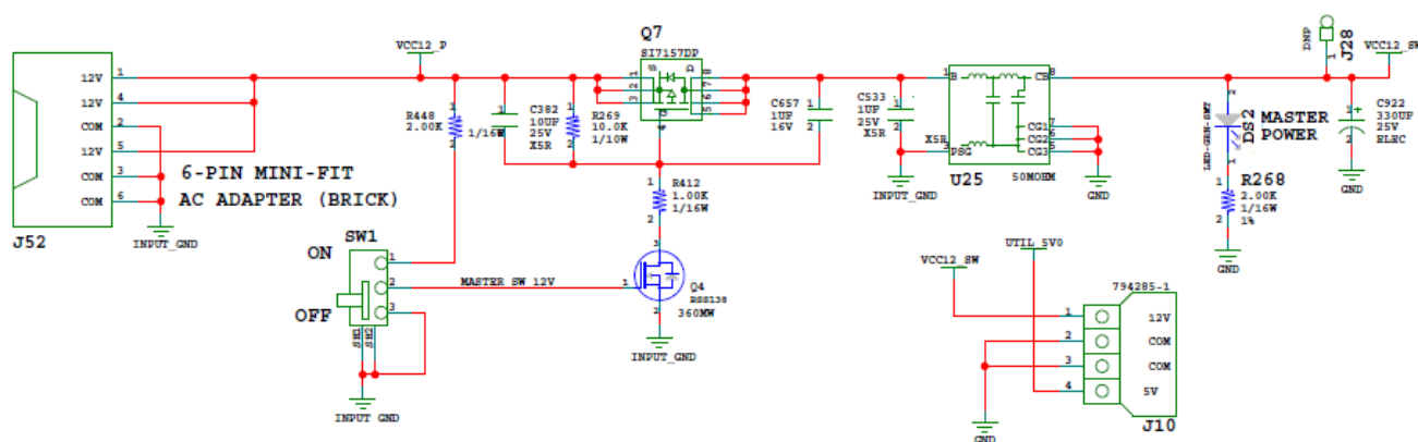
Figure 3-45: Power Input
