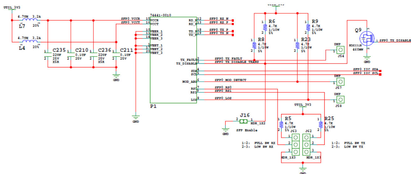
Figure 3-29: Typical SFP Interface
