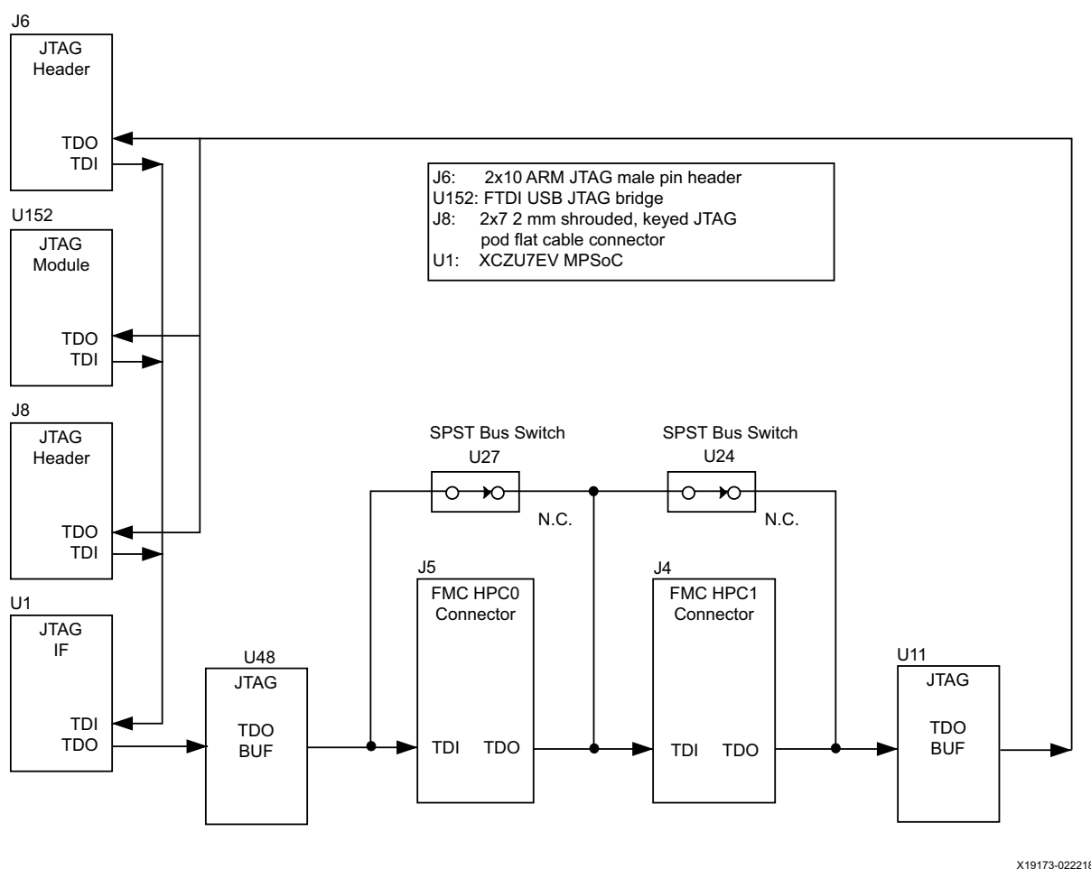
Figure 3-6: JTAG Chain Block Diagram
