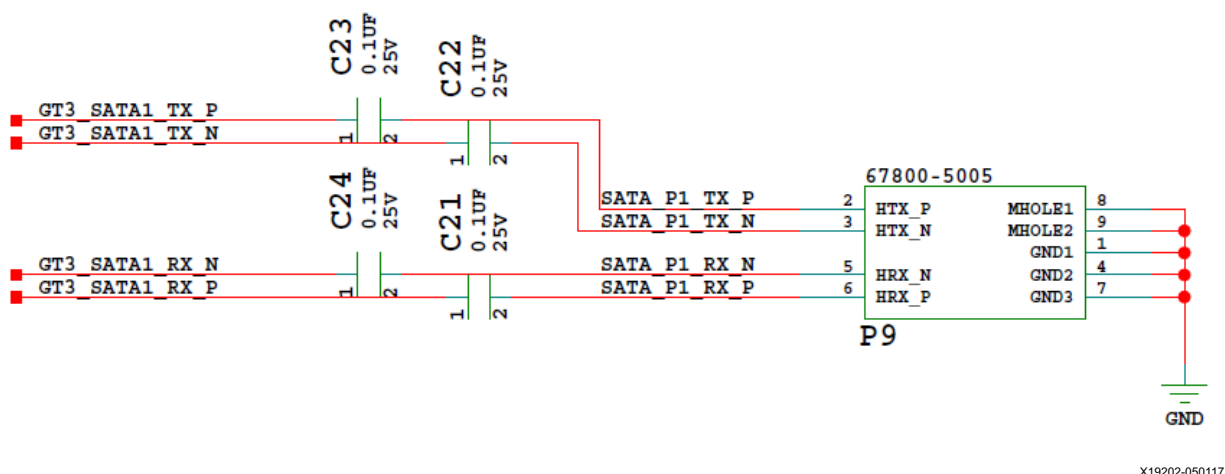
Figure 3-42: PS-GTR SATA
