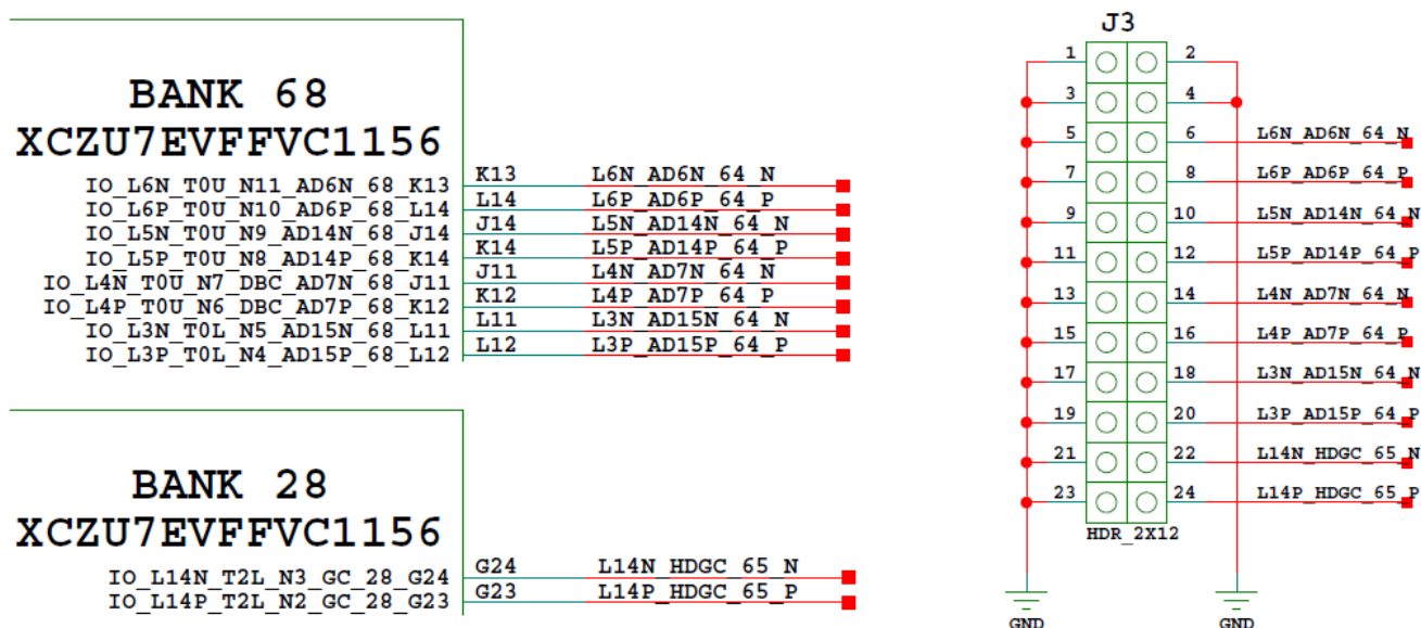
Figure 3-32: Prototype Header J3
