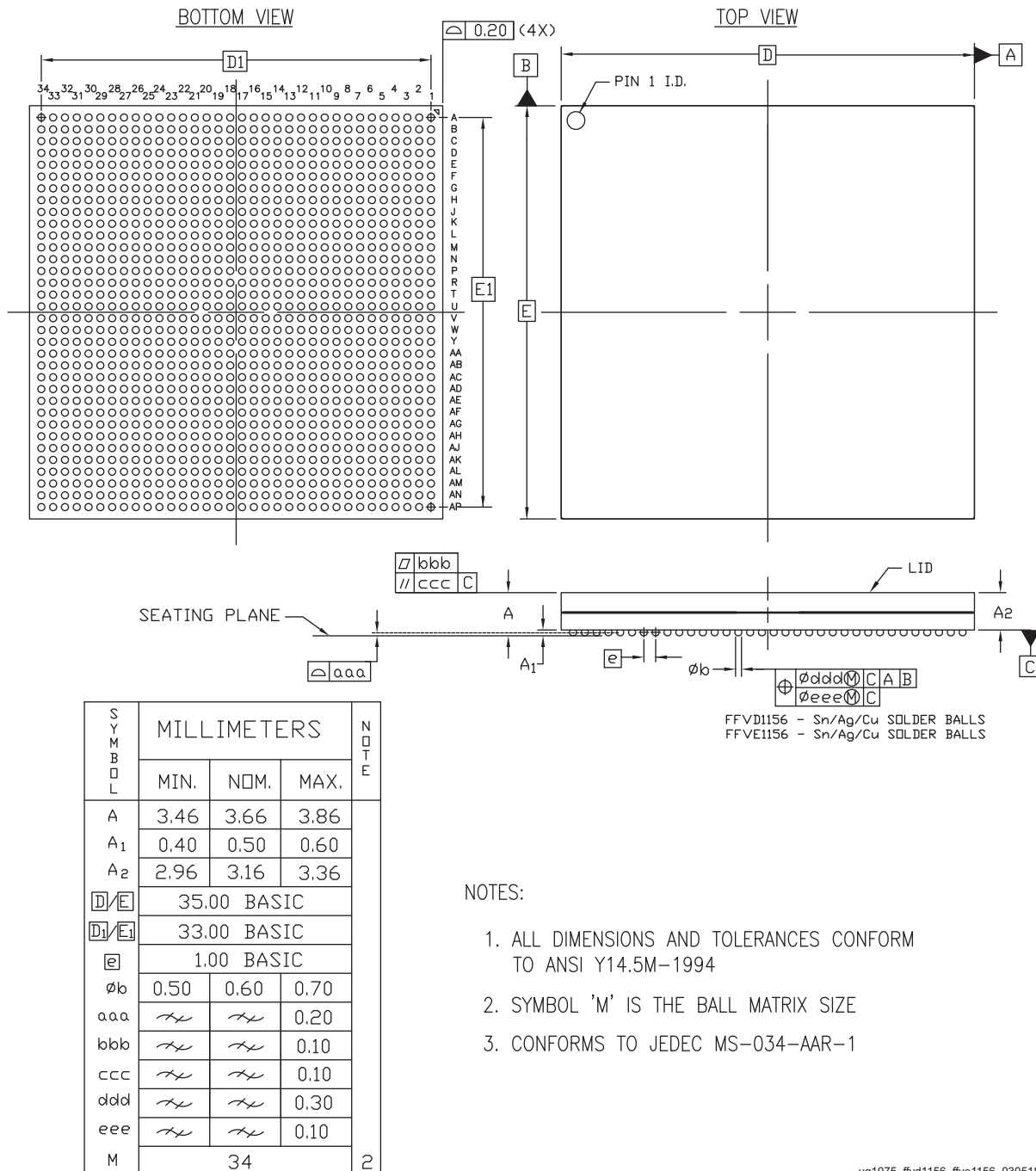
Figure 5-17: Package Dimensions for FFVD1156 (XCZU21DR) and FFVE1156 (XCZU25DR, XCZU27DR, XCZU28DR, XCZU43DR, XCZU47DR, XCZU48DR)
