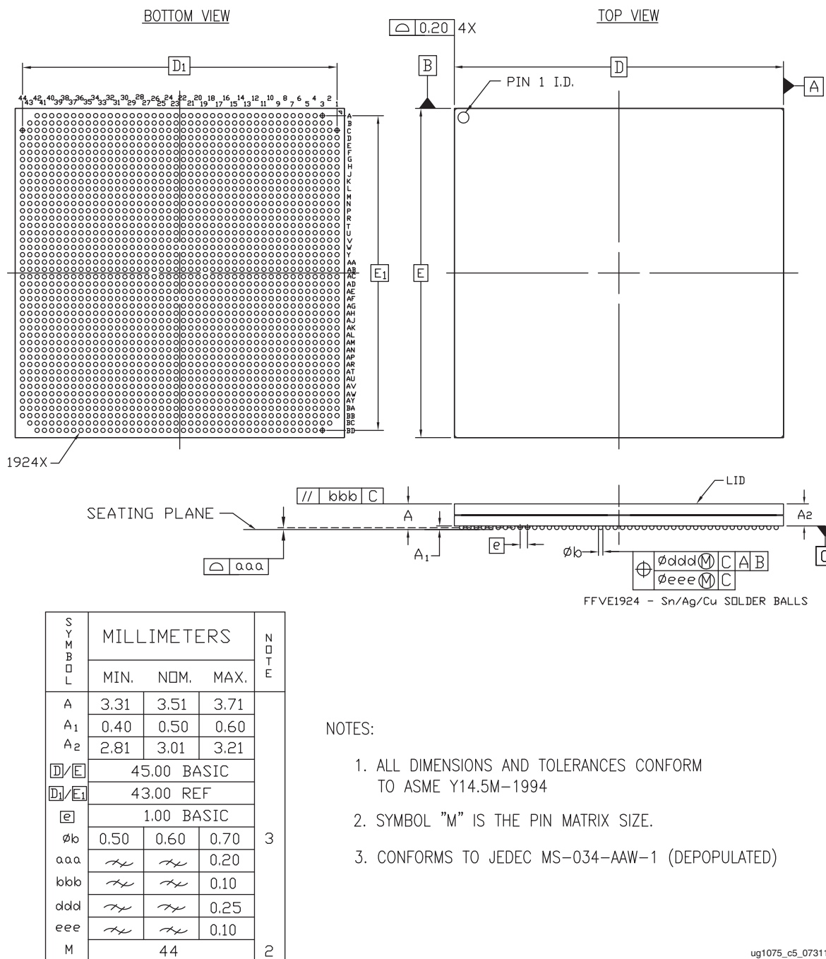
Figure 5-29: Package Dimensions for FFVE1924 (XCZU17EG and XCZU19EG)
