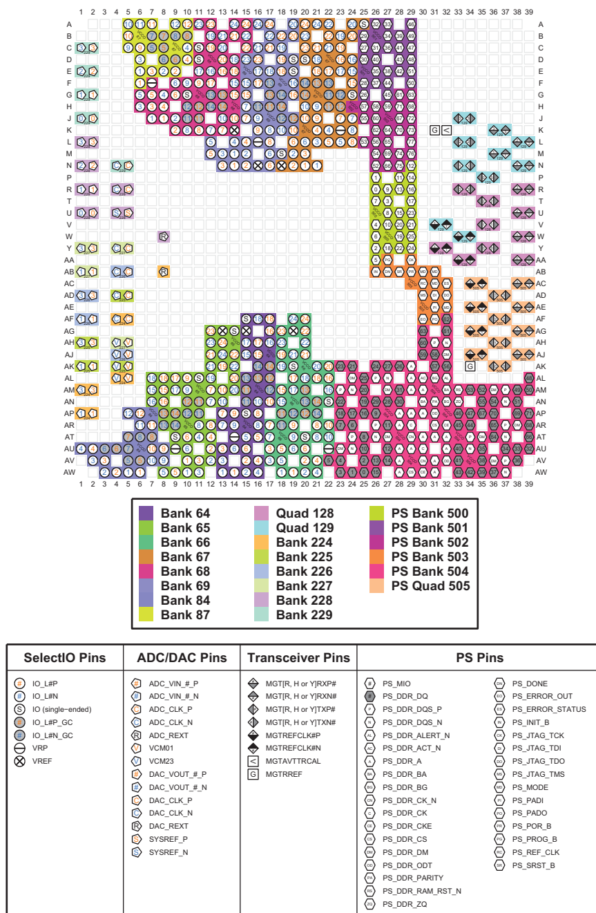
Figure 4-51: FFVG1517 and FSVG1517 Packages—XCZU25DR I/O Bank Diagram
