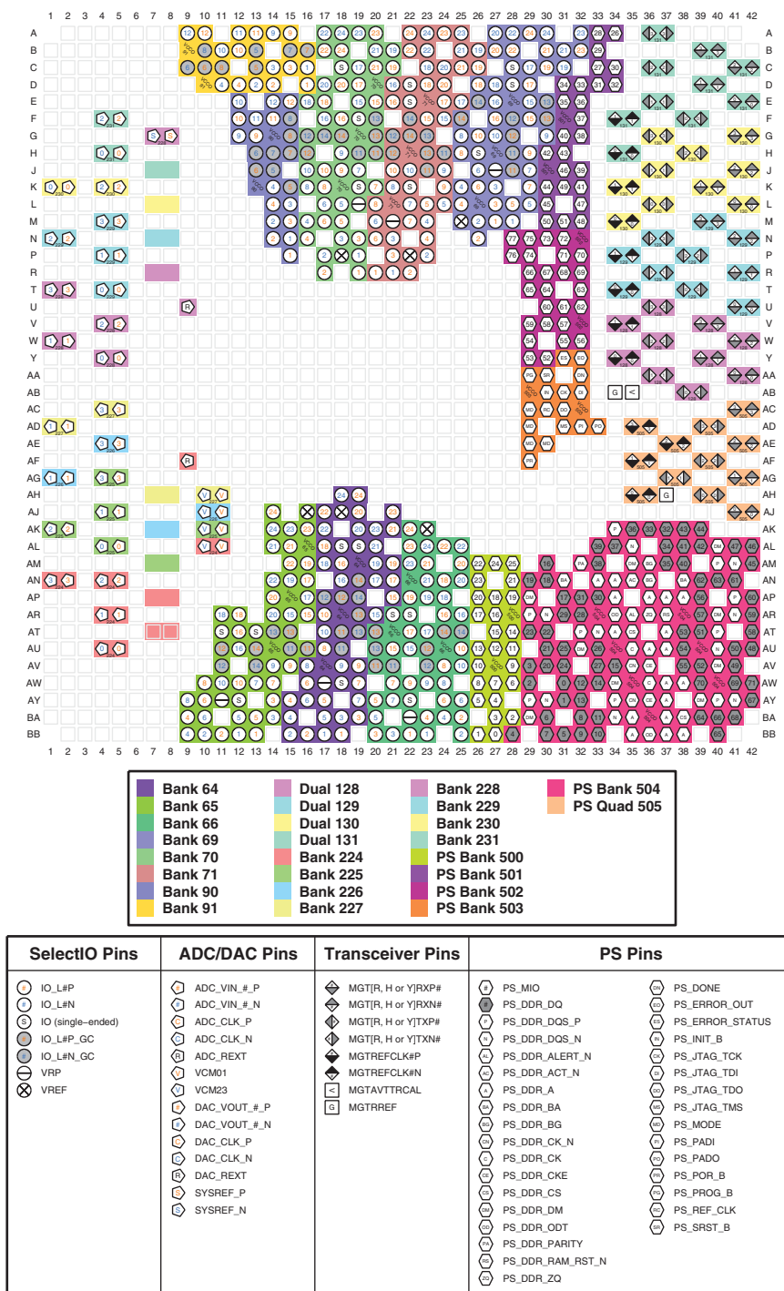
Figure 4-71: FFVH1760 and FSVH1760 Packages—XCZU49DR I/O Bank Diagram
