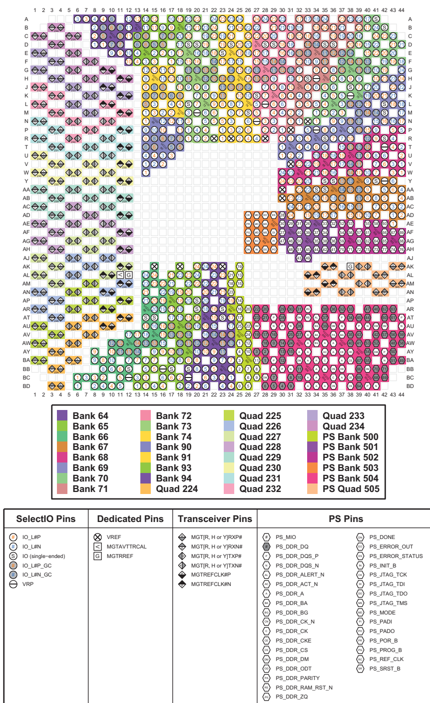
Figure 4-73: FFVE1924 Package—I/O Bank Diagram
