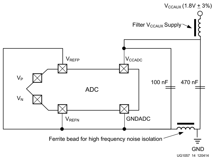
Figure 1-14: SYSMON On-chip Reference
