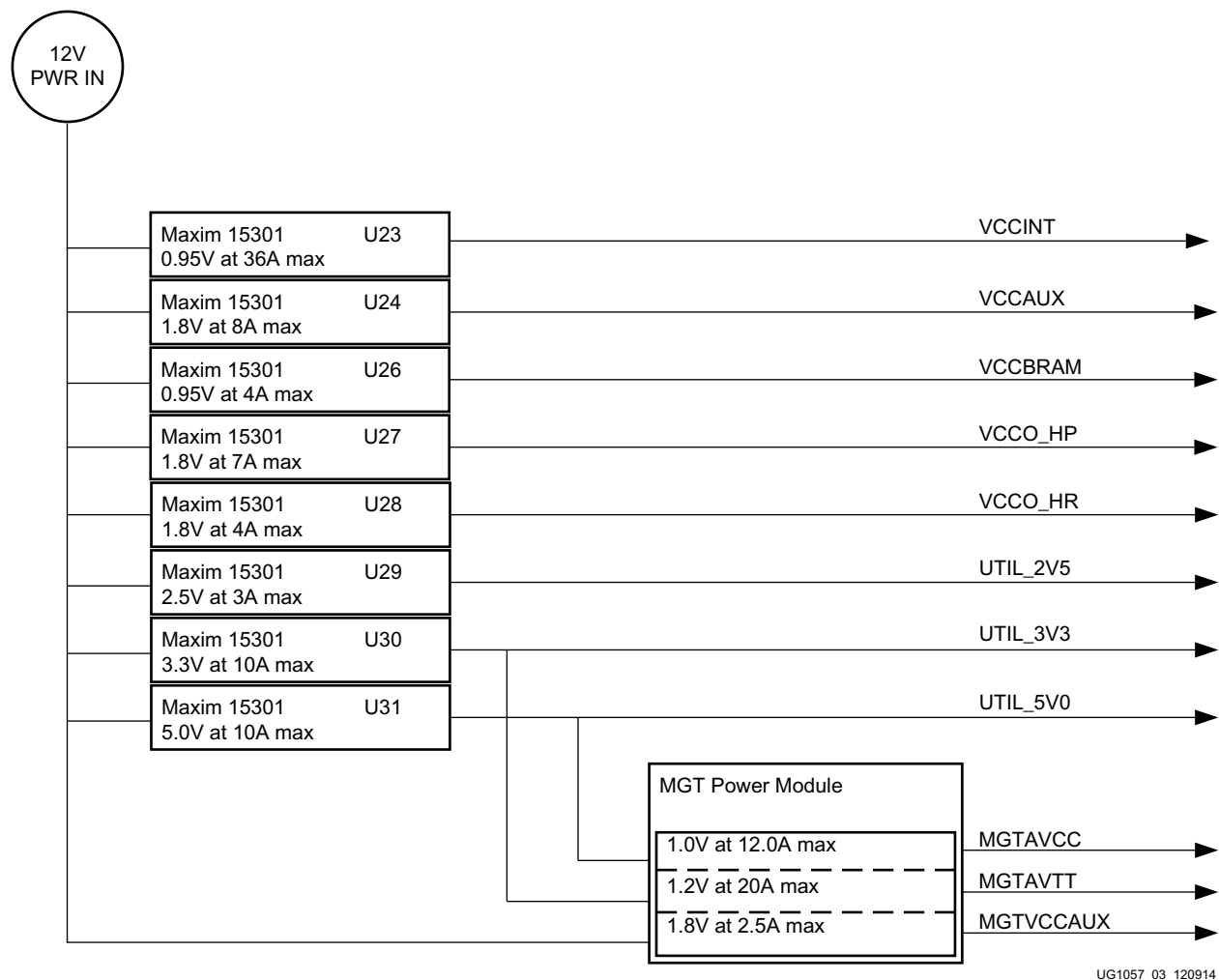
Figure 1-3: KCU1250 Board Power Supply Block Diagram
