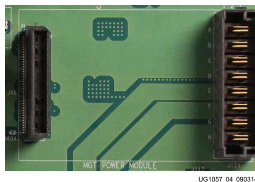
Figure 1-5: Mounting Location, MGT Power Module
