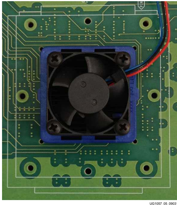
Figure 1-6: Active FPGA Heat Sink
