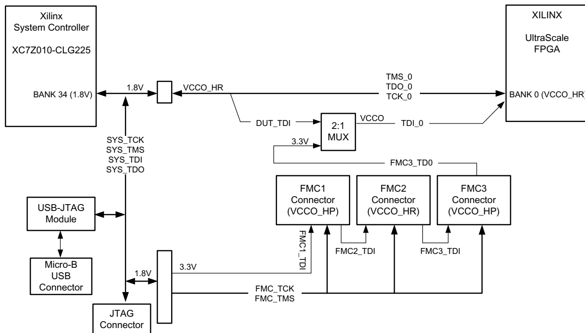
Figure 1-8: JTAG Chain
