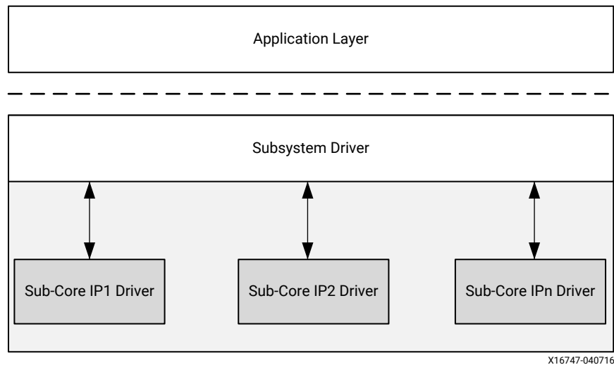
Figure 47: Subsystem Driver Architecture
