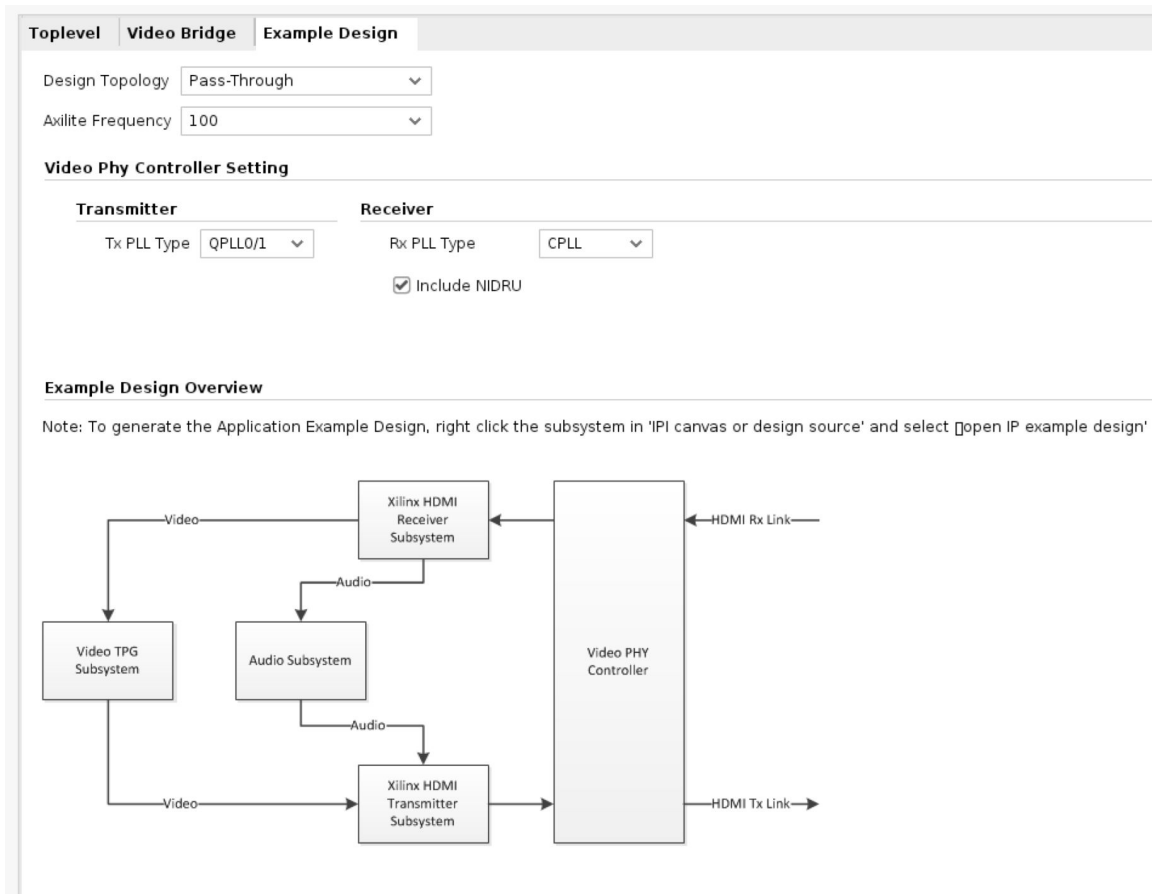
Figure 34: Example Design Tab
