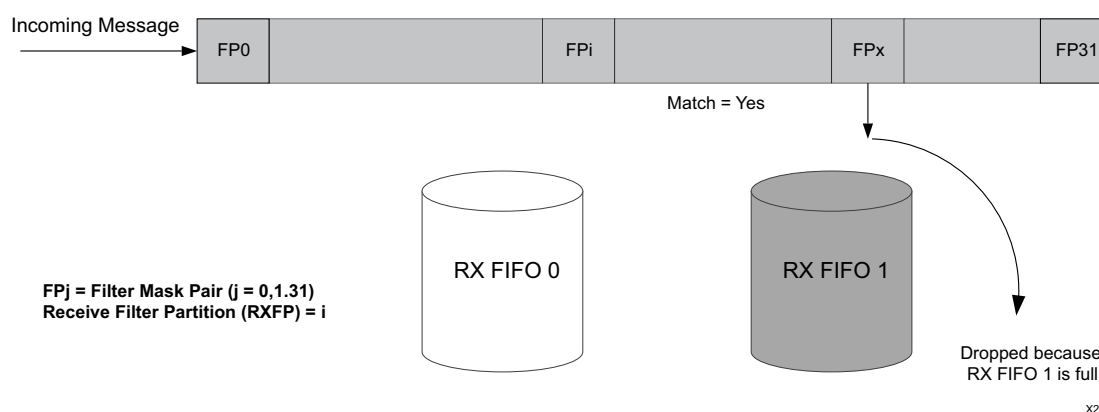
Figure 2-4: Message Drop (RX FIFO-1 Full and Match = Yes)
