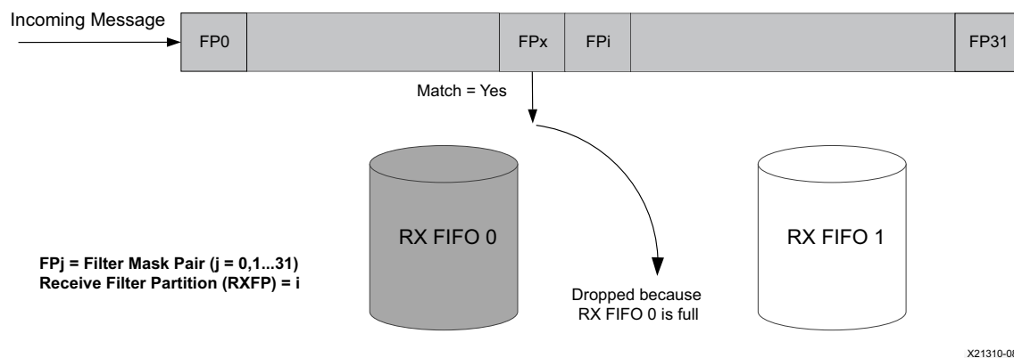
Figure 2-3: Message Drop (RX FIFO-0 Full and Match = Yes)
