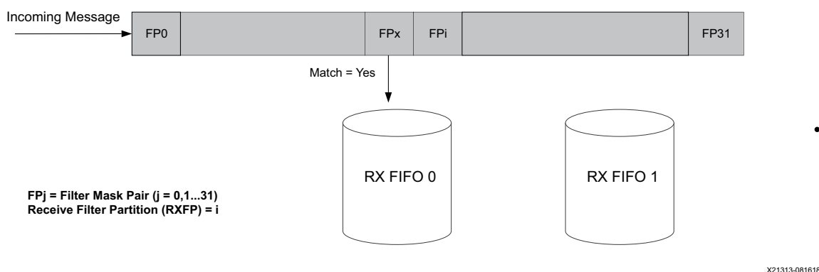
Figure 2-1: Normal Operation (RX FIFO-0)
