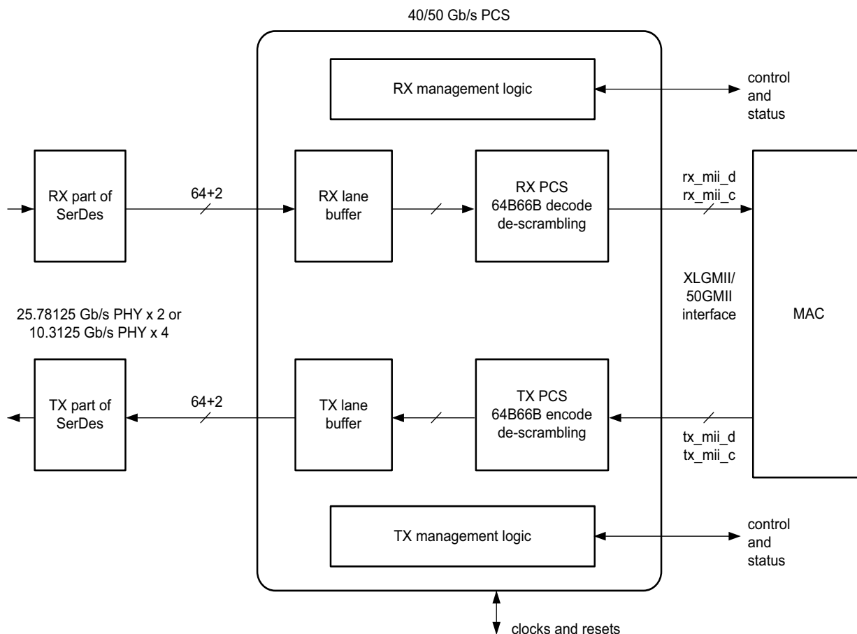
Figure 2-16: PCS Variant
