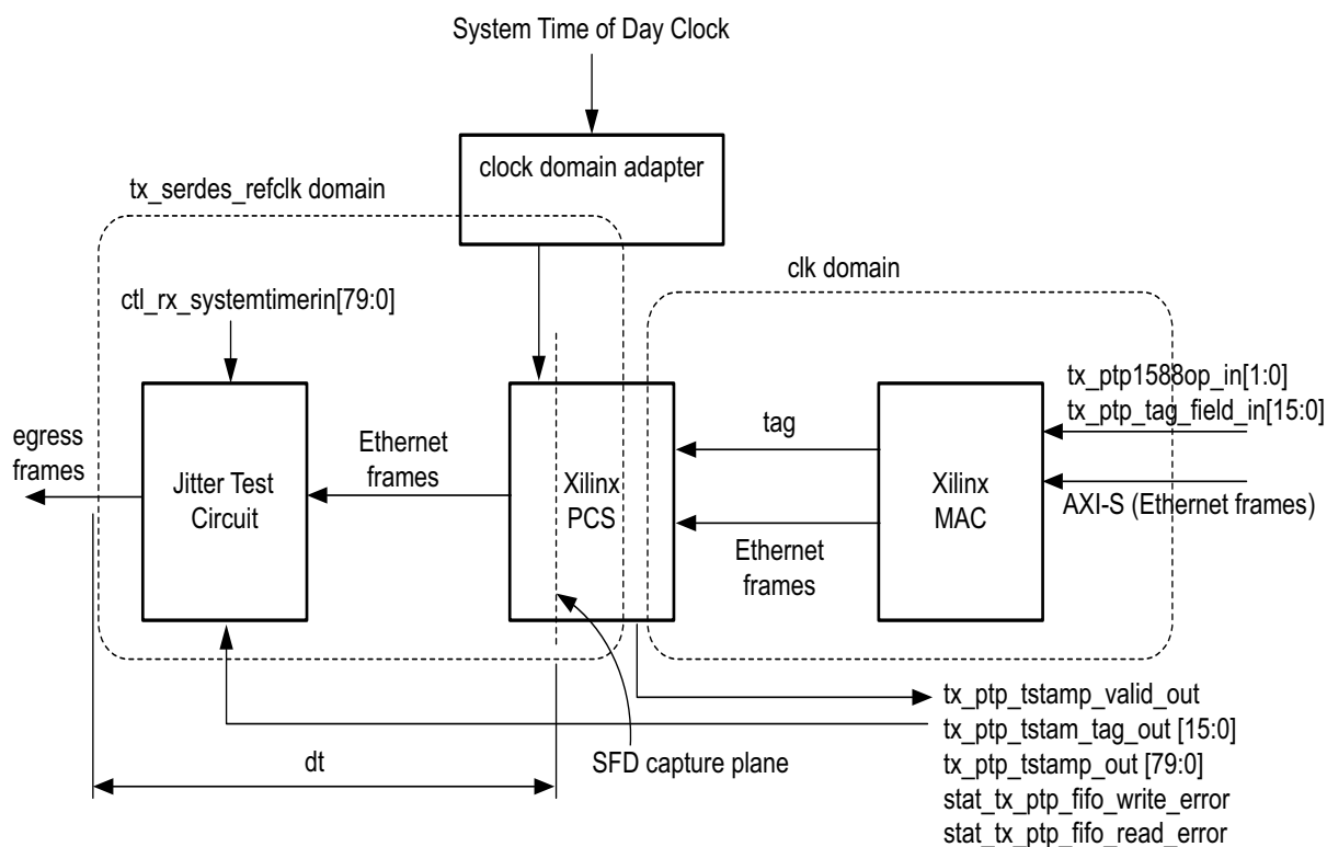
Figure 3-17: Transmit
