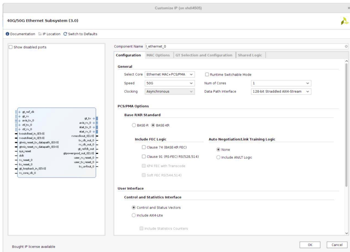
Figure 4-1: Configuration Tab
