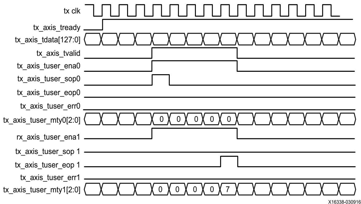
Figure 2-6: TX Waveform
