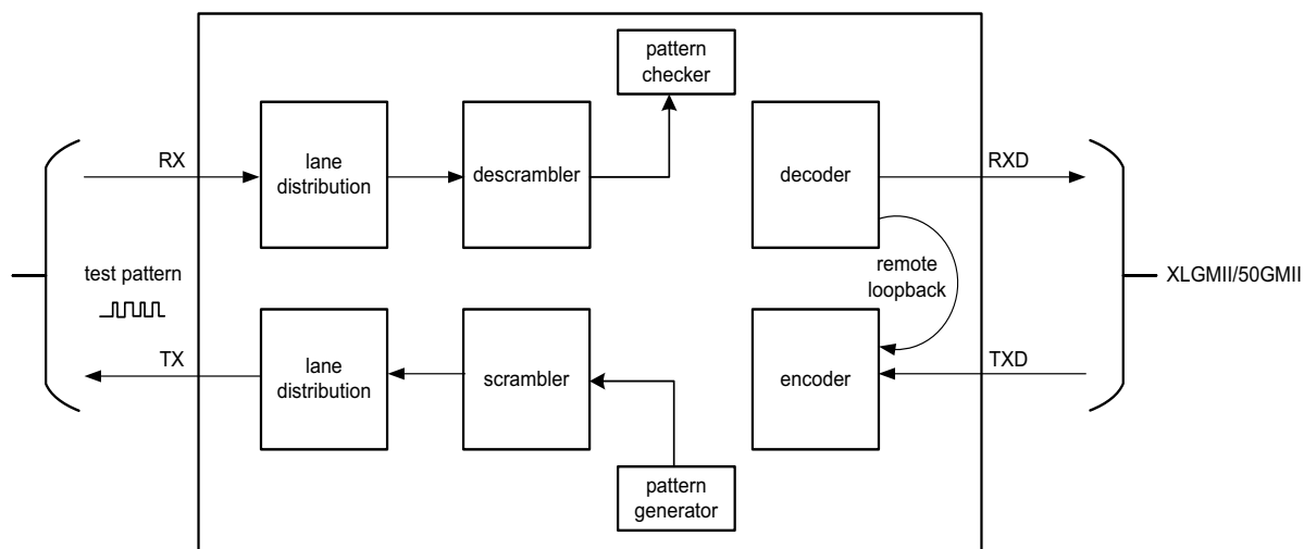
Figure 2-17: PCS Loopback
