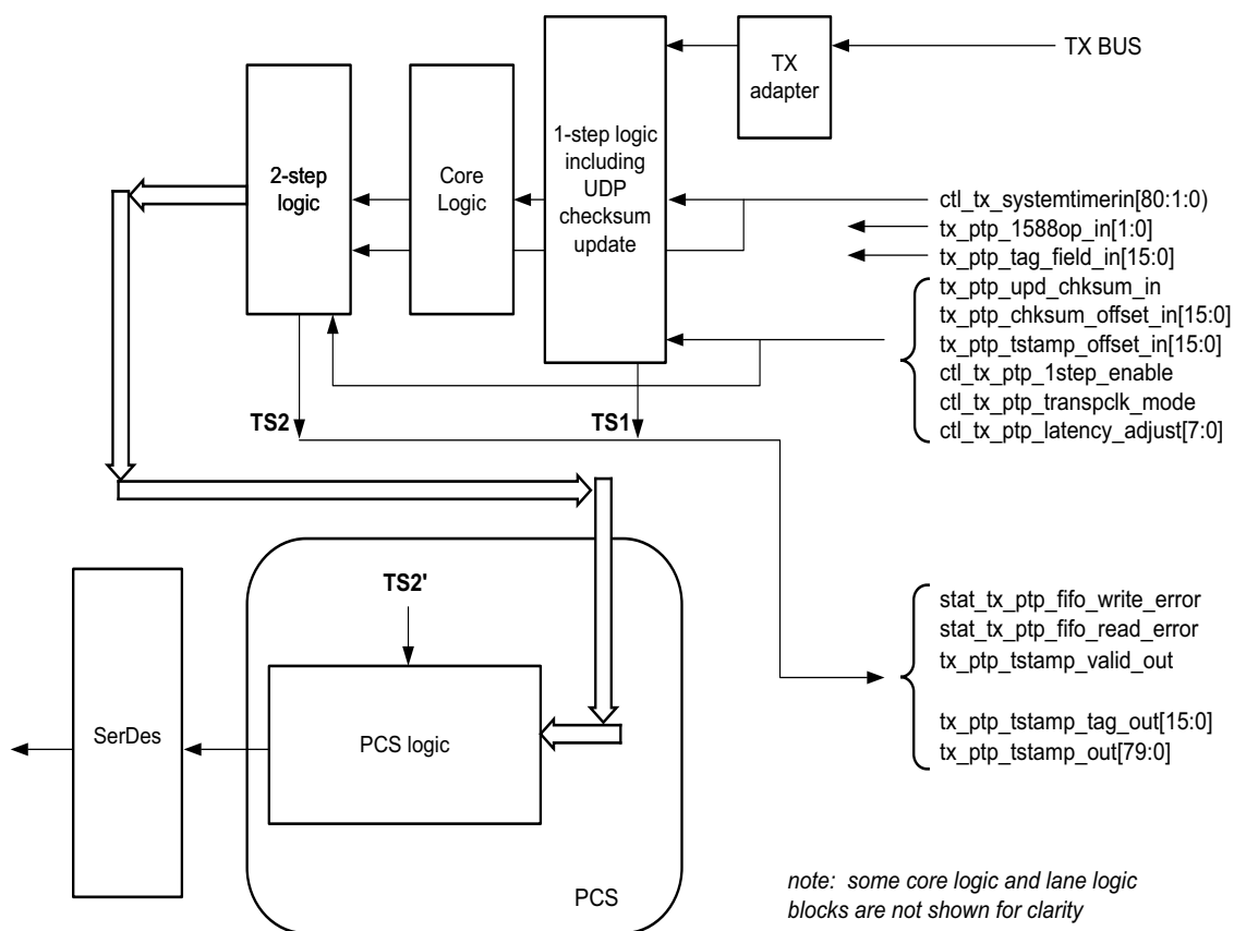
Figure 3-14: Egress
