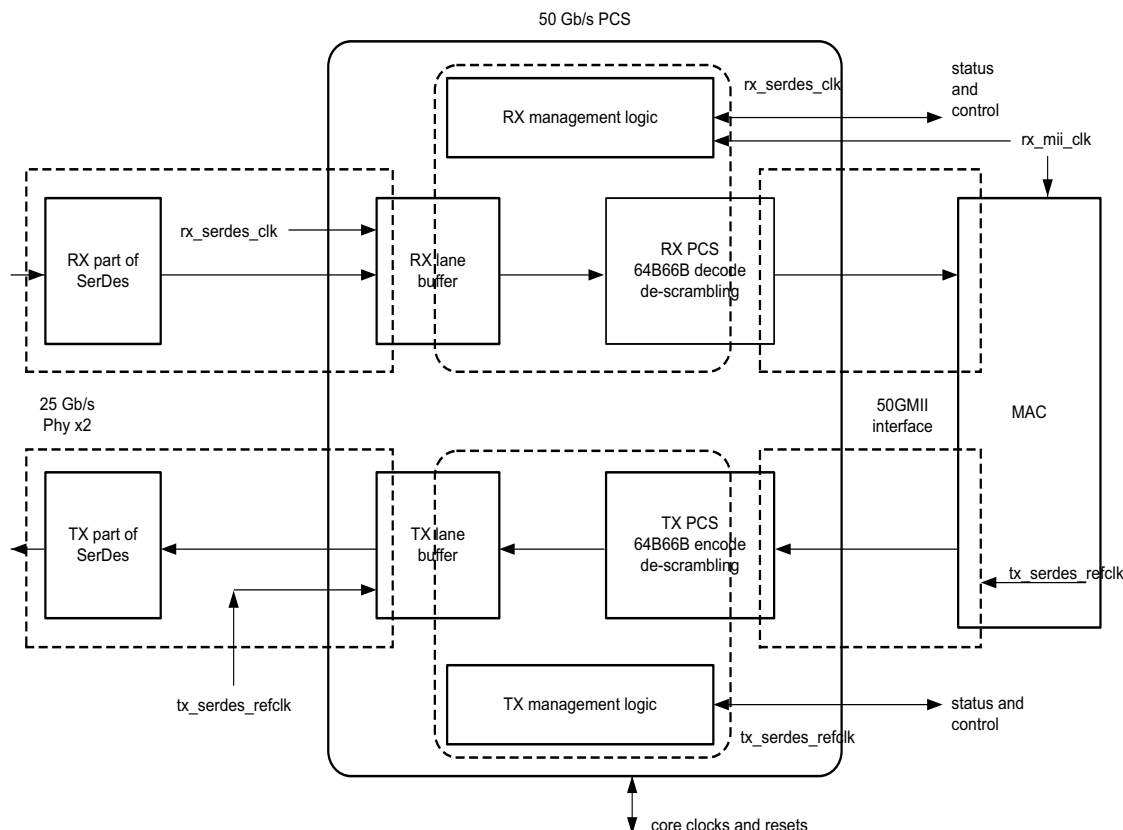
Figure 2-18: PCS Clocking
