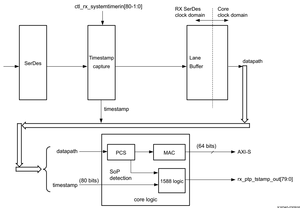
Figure 3-15: Ingress
