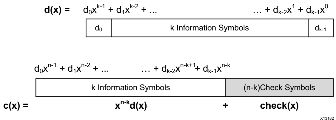
Figure 2-1: Reed Solomon Codeword Structure
