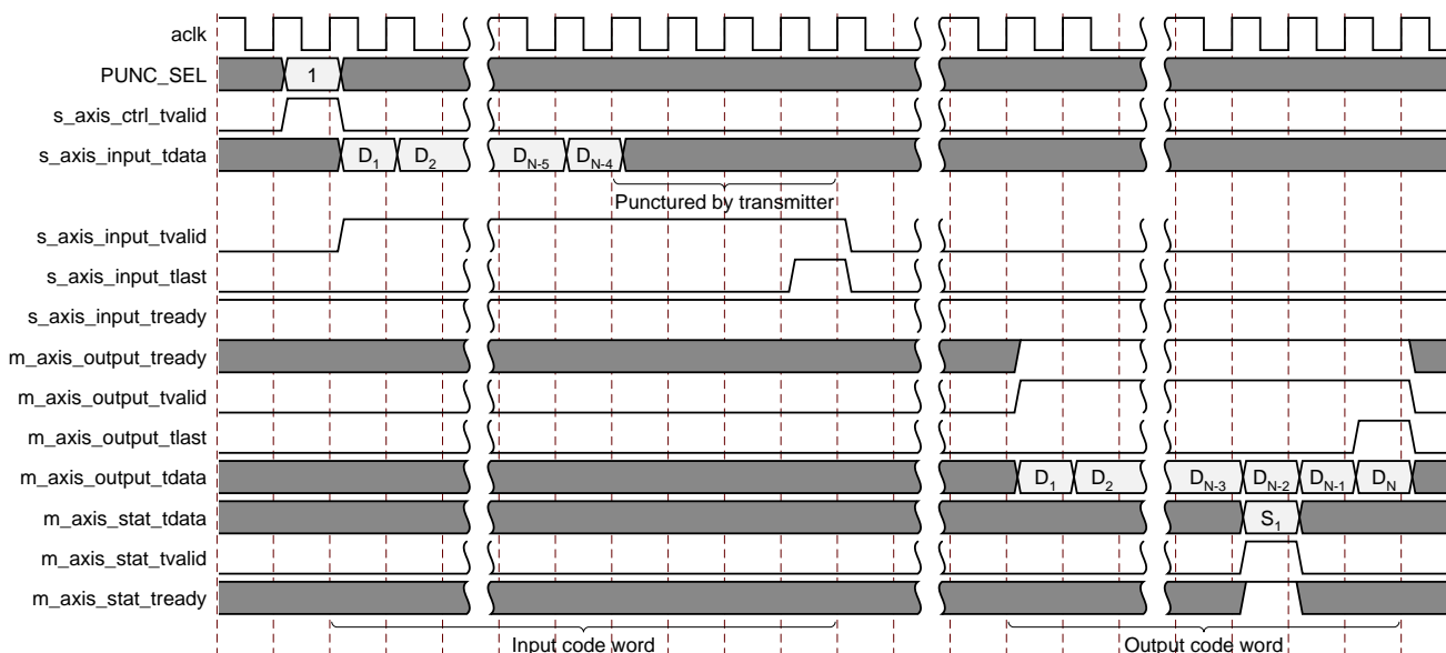
Figure 3-13: Puncture Timing
