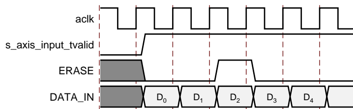
Figure 3-10: ERASE Timing
