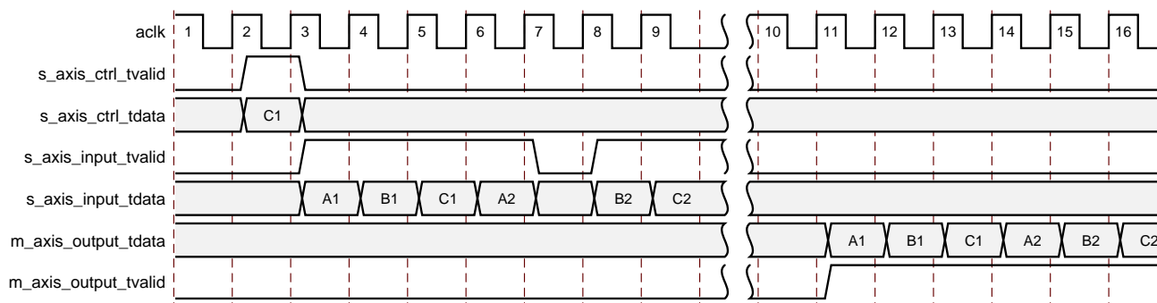
Figure 3-16: Multi-Channel Operation
