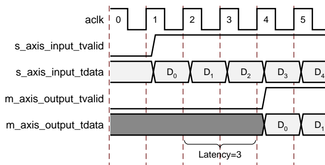
Figure 3-12: Latency = 3
