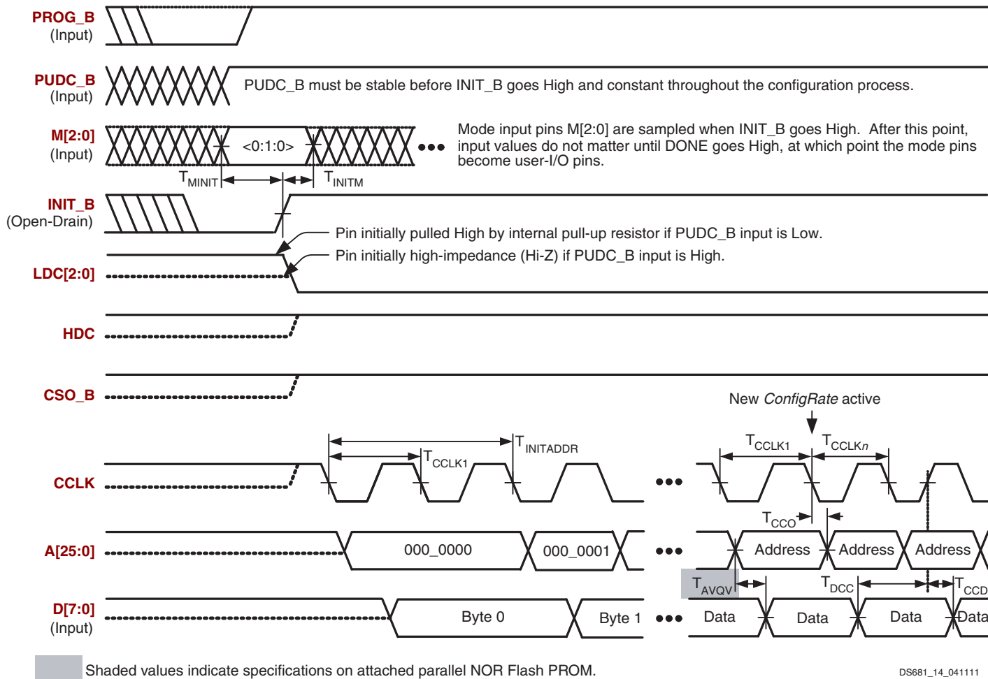
Figure 15: Waveforms for BPI Configuration
