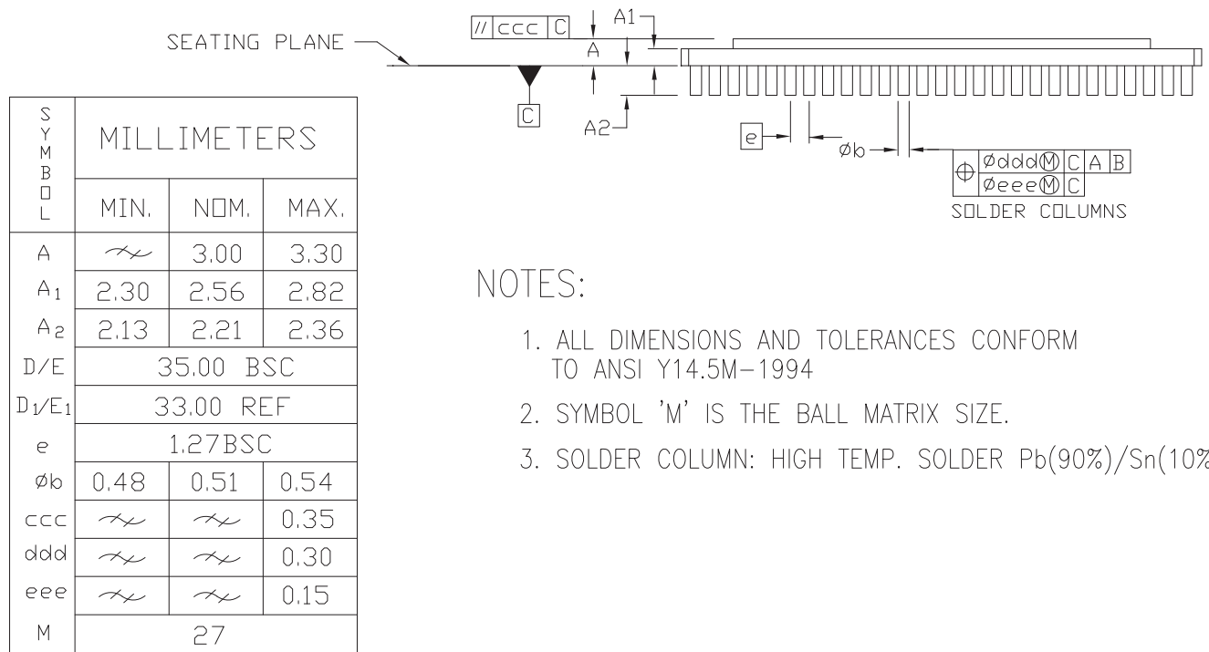
Figure 54: CG717 Ceramic CGA Package Specifications
