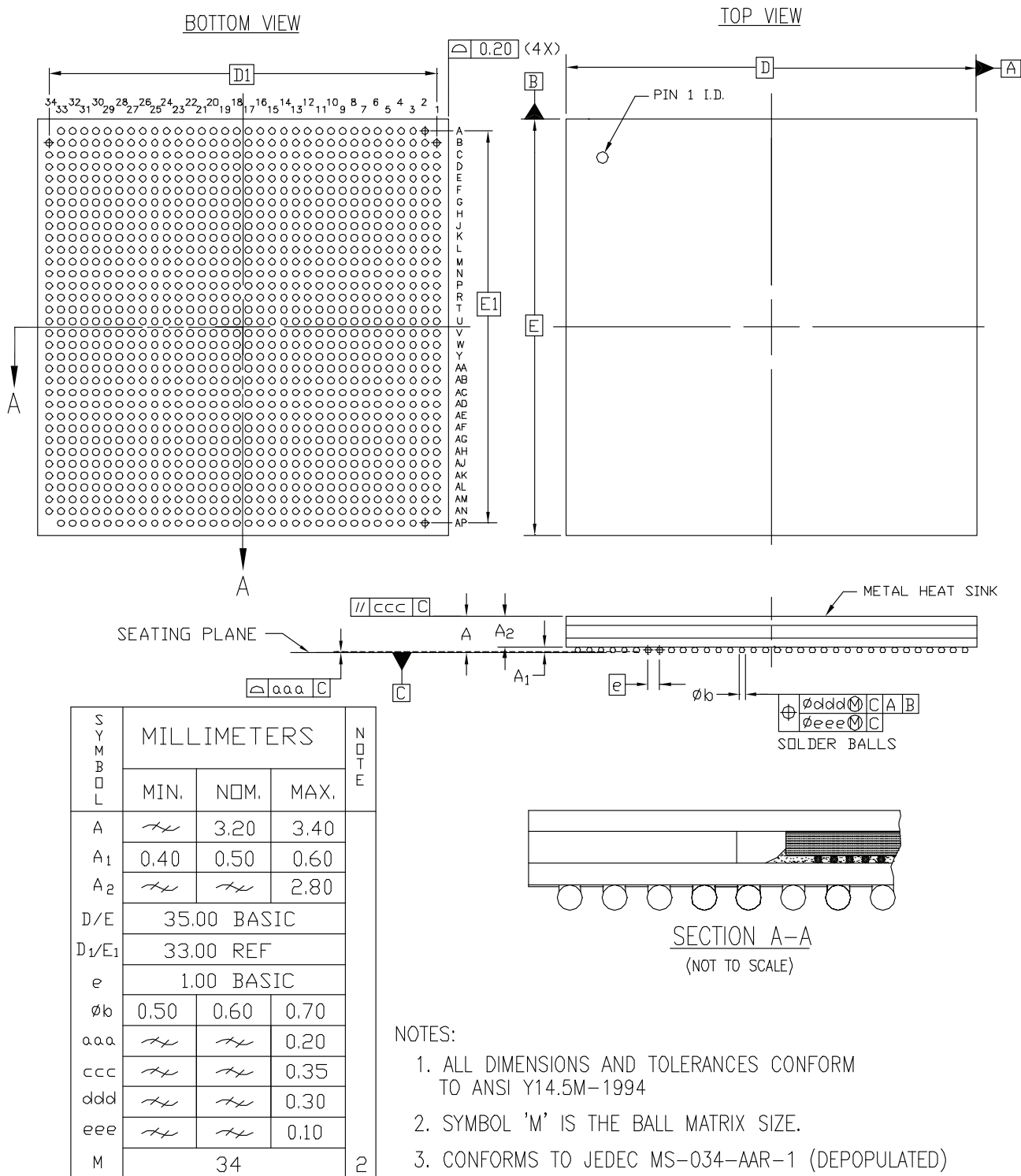
Figure 57: EF1152 Epoxy-Coated Flip-Chip BGA Package Specifications
