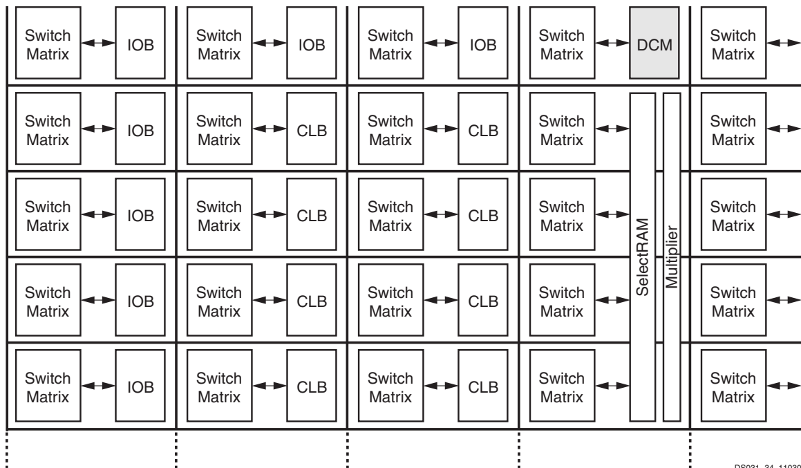
Figure 49: Routing Resources
