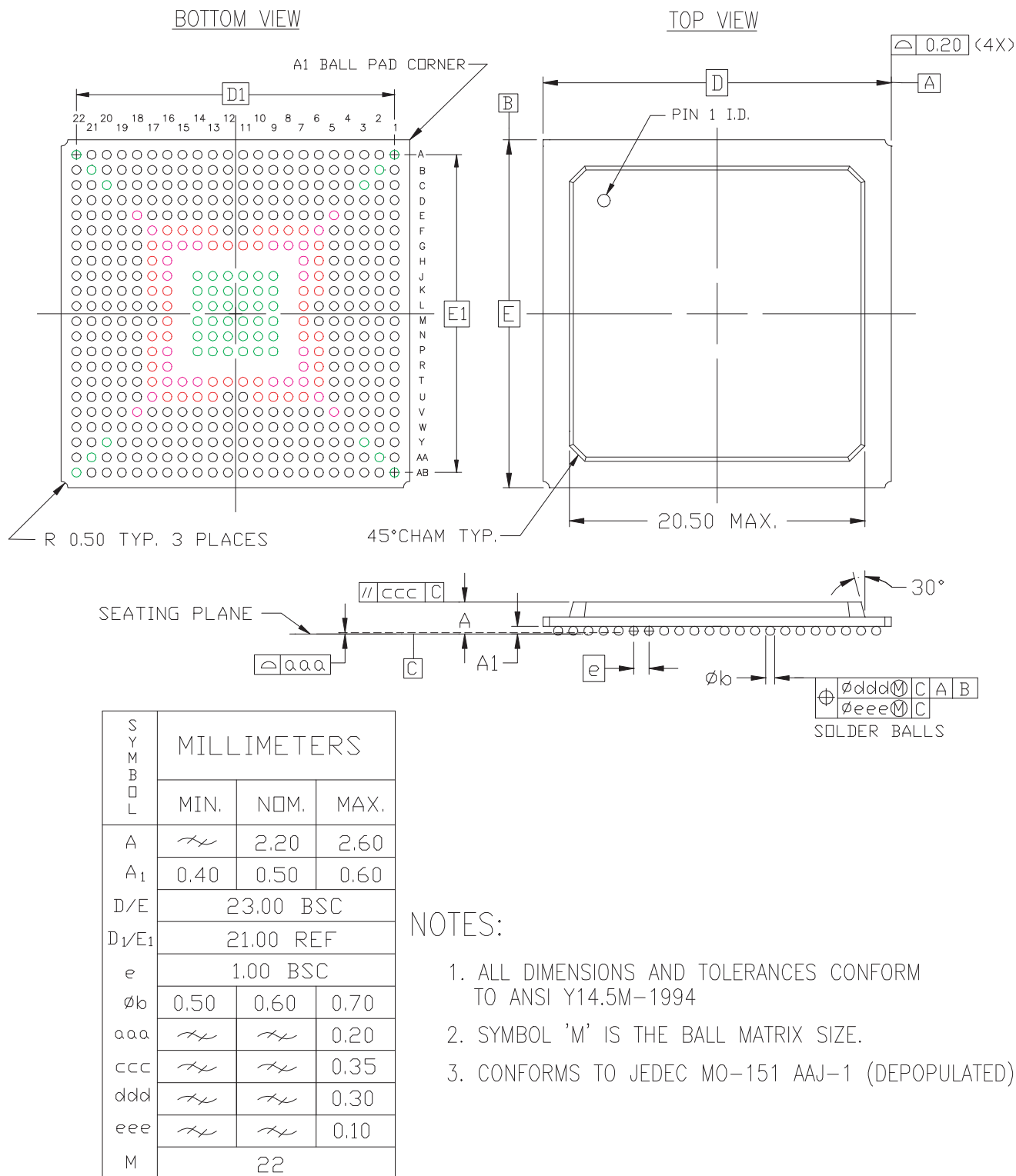
Figure 51: FG456 Fine-Pitch BGA Package Specifications
