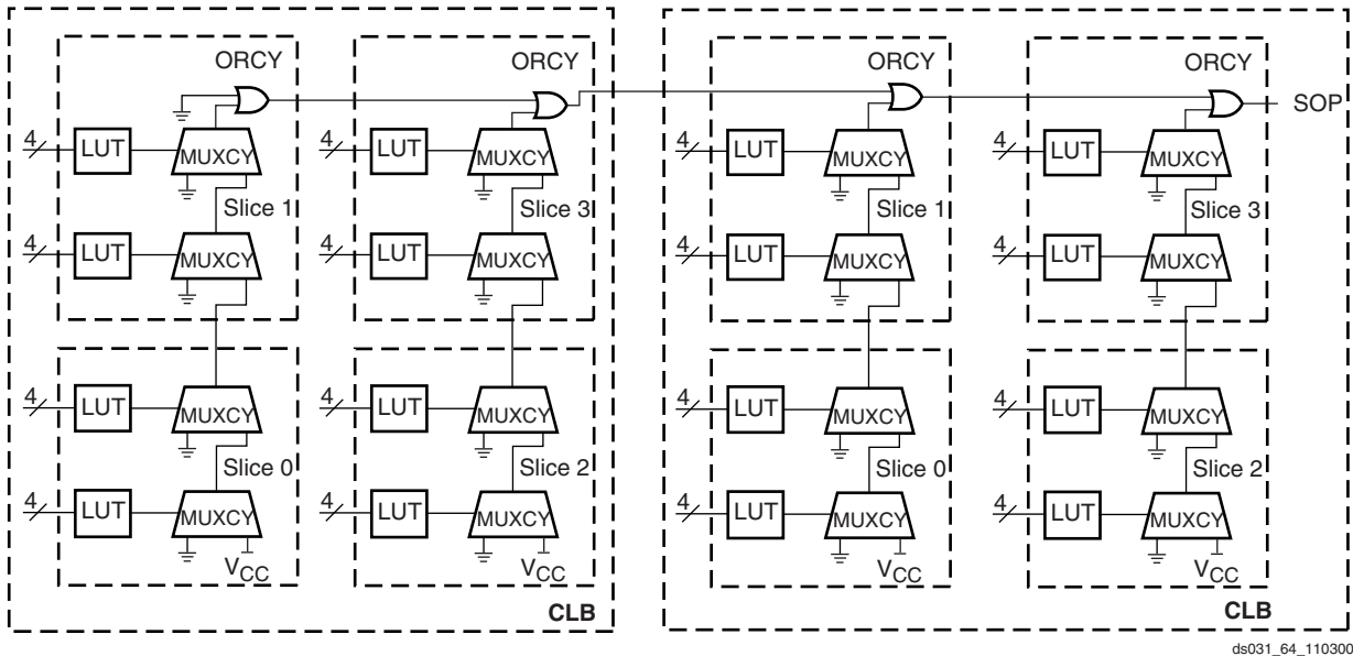
Figure 26: Horizontal Cascade Chain
