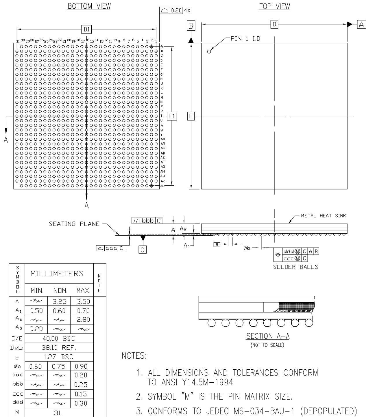
Figure 55: EF957 Epoxy-Coated Flip-Chip BGA Package Specifications
