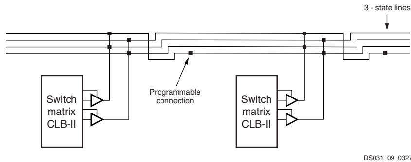
Figure 29: 3-State Buffer Connection to Horizontal Lines
