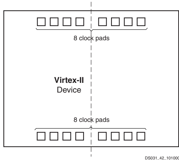
Figure 39: Virtex-II Clock Pads
