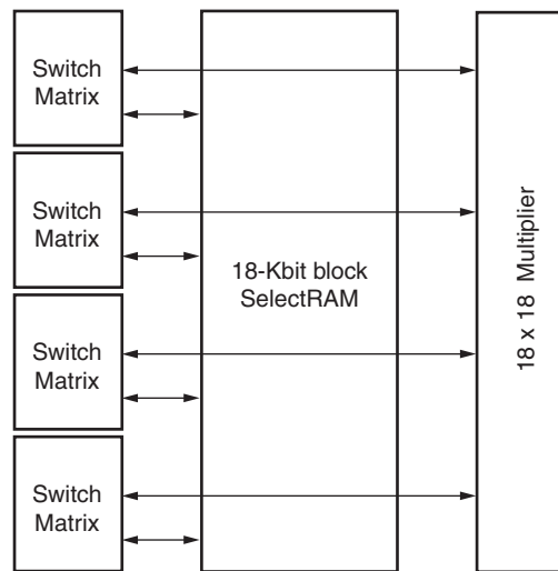
Figure 36: SelectRAM and Multiplier Blocks
