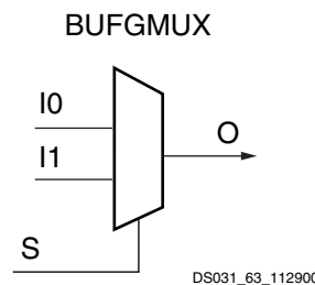
Figure 44: Virtex-II BUFGMUX Function
