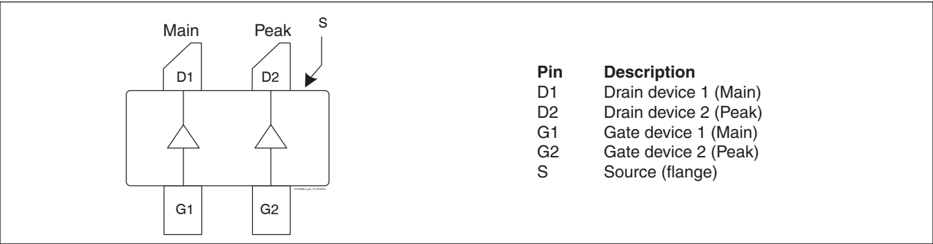
Lead connections for PTRA094252FC
