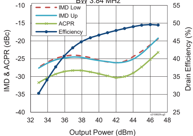
Two-carrier WCDMA Drive-up V_{DD} = 28\text{ V} , I_{DQ} = 100\text{ mA} , V_{GS1} = 1.3\text{ V} , f = 2170\text{ MHz} , 3GPP WCDMA signal, PAR = 8 dB, 10 MHz carrier spacing, BW 3.84 MHz
