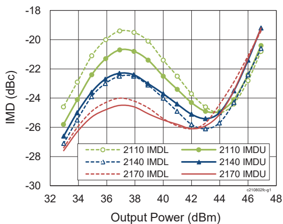
Two-carrier WCDMA Drive-up V_{DD} = 28\text{ V} , I_{DQ} = 100\text{ mA} , V_{GS1} = 1.3\text{ V} , 3GPP WCDMA signal, PAR = 8 dB, 10 MHz carrier spacing, BW 3.84 MHz
