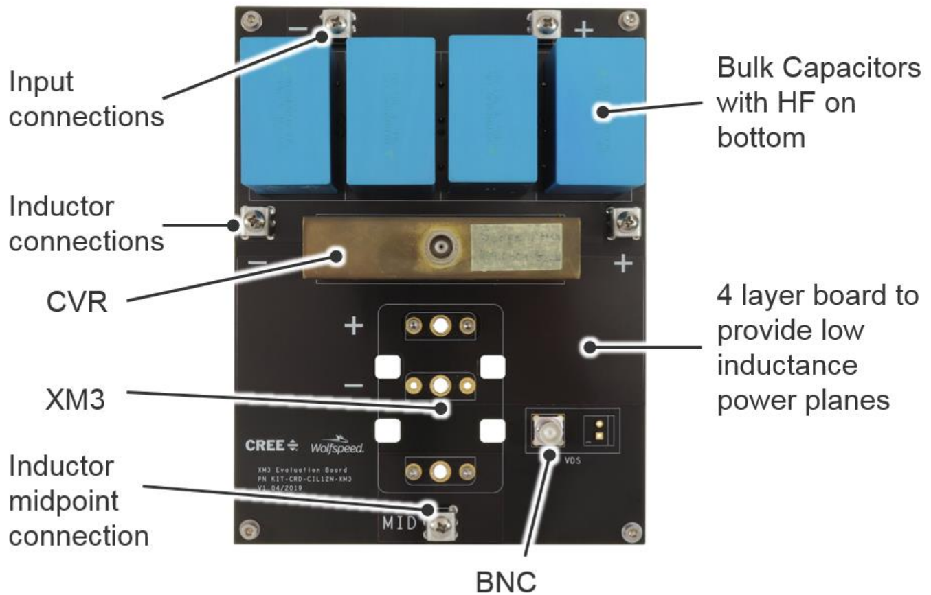
Figure 4 Evaluation Board
