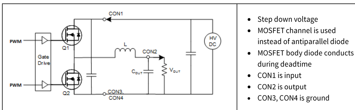
Figure 3. Cree's KIT-CRD-8FF65P/CRD-8FF90P Evaluation Kit configured as Synchronous Buck Converter
