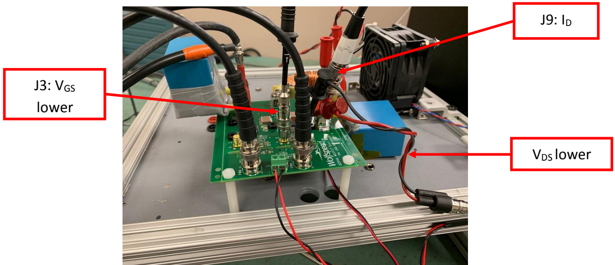
Figure 18. Probe Locations
