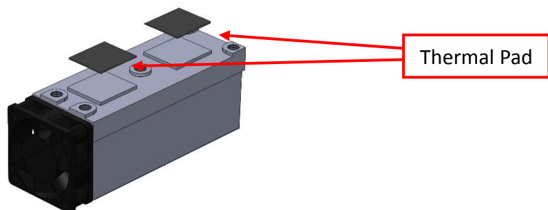
Figure 8. Thermal Gap Filler Pad
