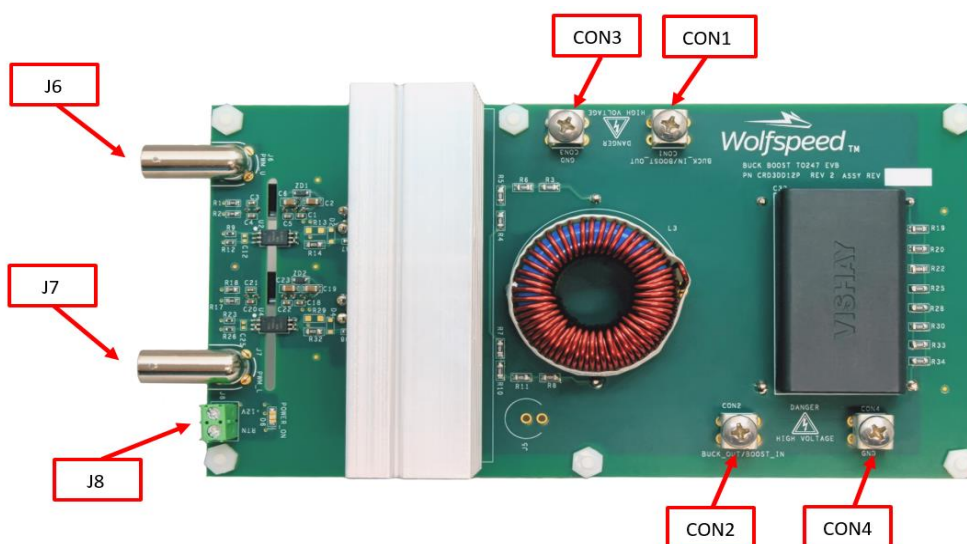
Figure 10. Terminals and Connections of Cree's KIT-CRD-3DD065P/CRD-3DD12P Buck-Boost Evaluation kit
