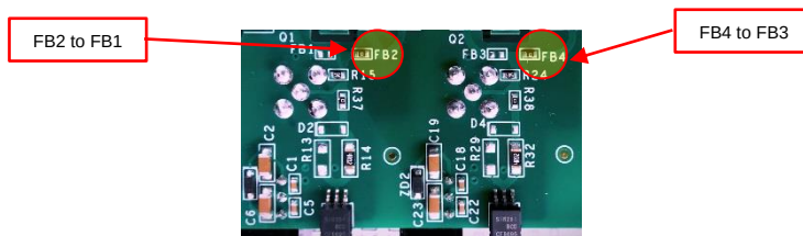
Figure 15. Location of Resistors on the top side of PCB
