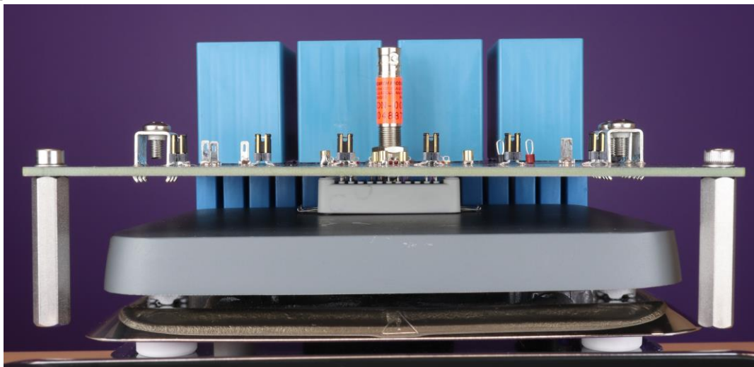
Figure 13. FM3 Module on Hot Plate for Elevated Temperature Testing
