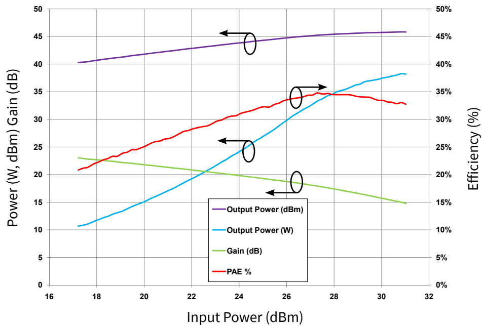
Figure 3. - Output Power, Gain and Power Added Efficiency vs. Input Power V_{DD} = 28\text{ V} , I_{DQ} = 1.2\text{ A} , Frequency = 11 GHz
