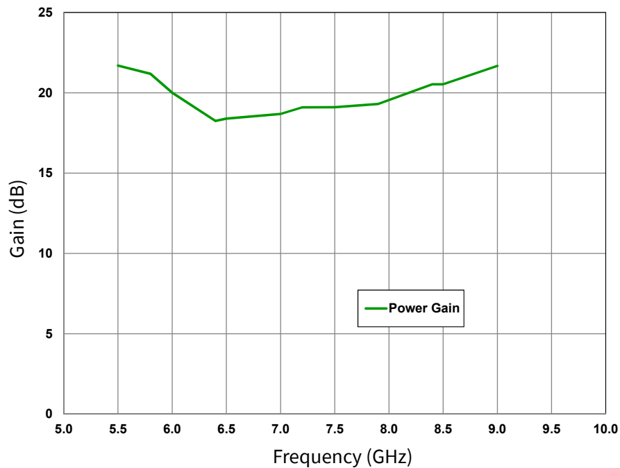
Figure 10. Gain @ Saturated Power vs. Frequency V_{DD} = 28\text{ V} , I_{DQ} = 800\text{ mA} , Pulsed Width = 100\text{ }\mu\text{s} , Duty Cycle = 10%
