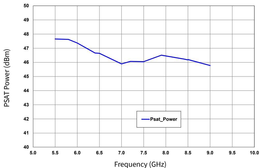
Figure 8. PSAT Power vs. Frequency
