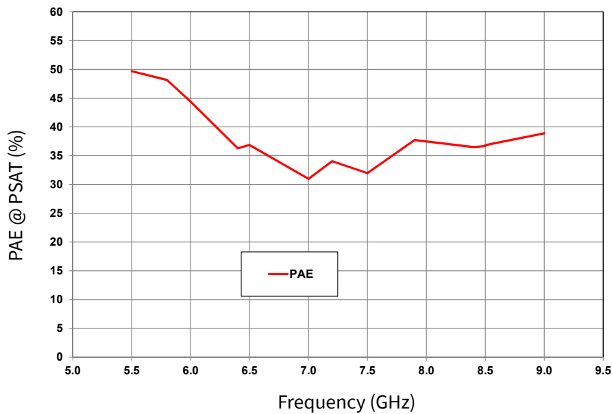
Figure 9. Power Added Efficiency @ Saturated Power vs. Frequency V_{DD} = 28\text{ V} , I_{DQ} = 800\text{ mA} , Pulsed Width = 100\text{ }\mu\text{s} , Duty Cycle = 10%
