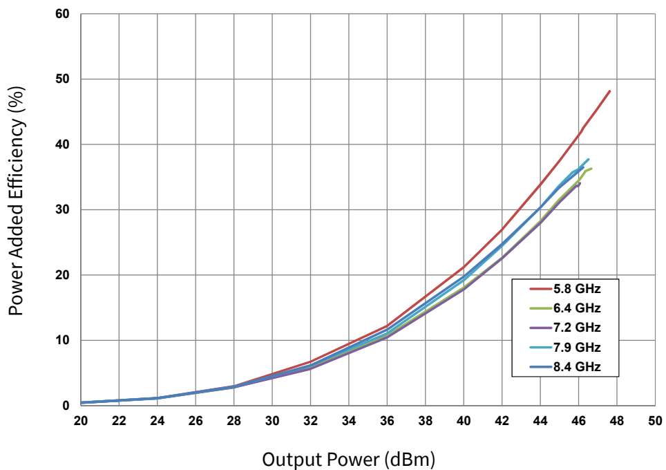
Figure 11. PAE vs. Output Power and Frequency
