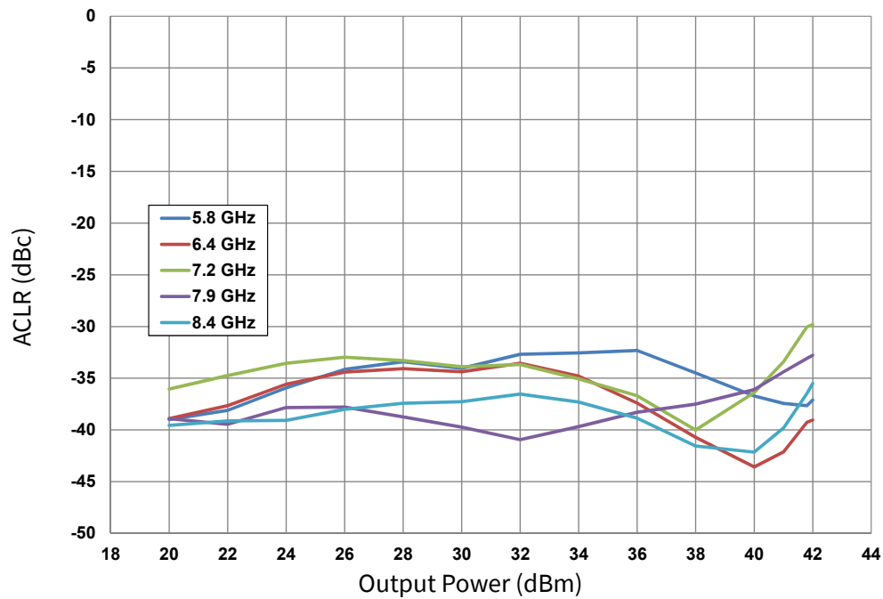
Figure 7. ACLR vs. Output Power and Frequency OQPSK 1.6 Msps
