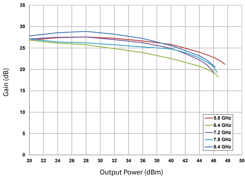
Figure 12. Gain vs. Output Power and Frequency
