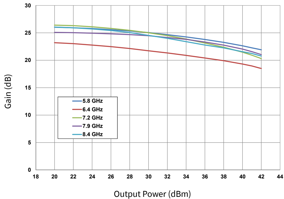
Figure 5. Gain vs. Output Power and Frequency OQPSK 1.6 Msps
