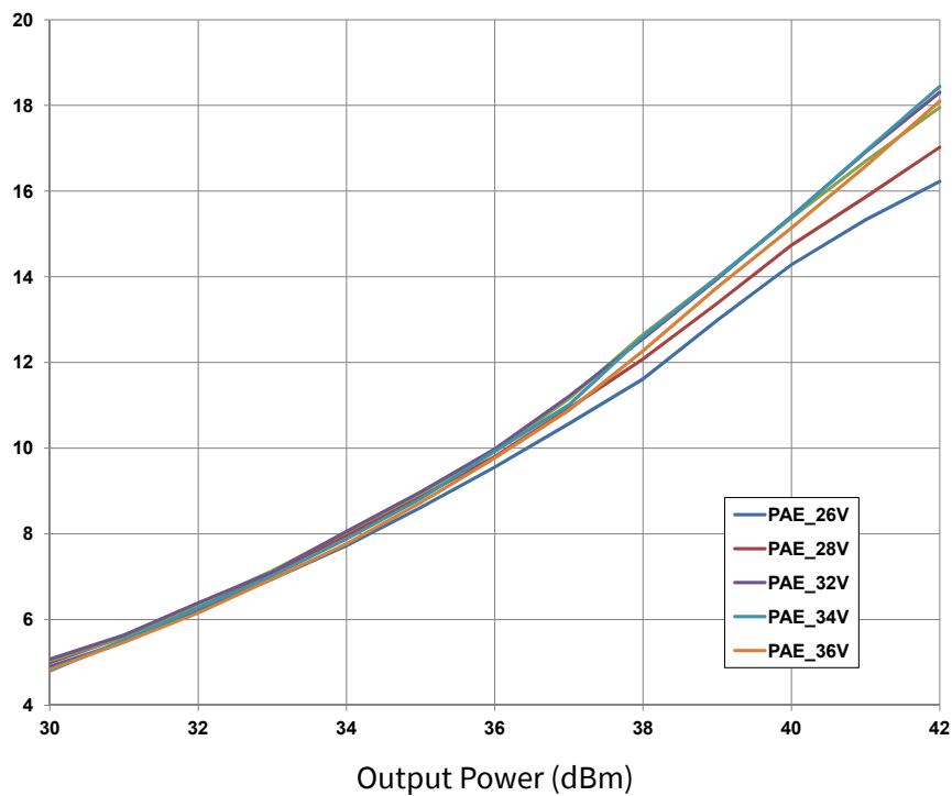
Figure 16. CPA1D1E025F Modulated Power Sweep (PAE and Gp) 1.6 Msps OQPSK Modulation, Frequency = 14 GHz V_{DD} = 26-36V , I_{DQ} = 150\text{ mA} , T_{case} = 25^{\circ}C
