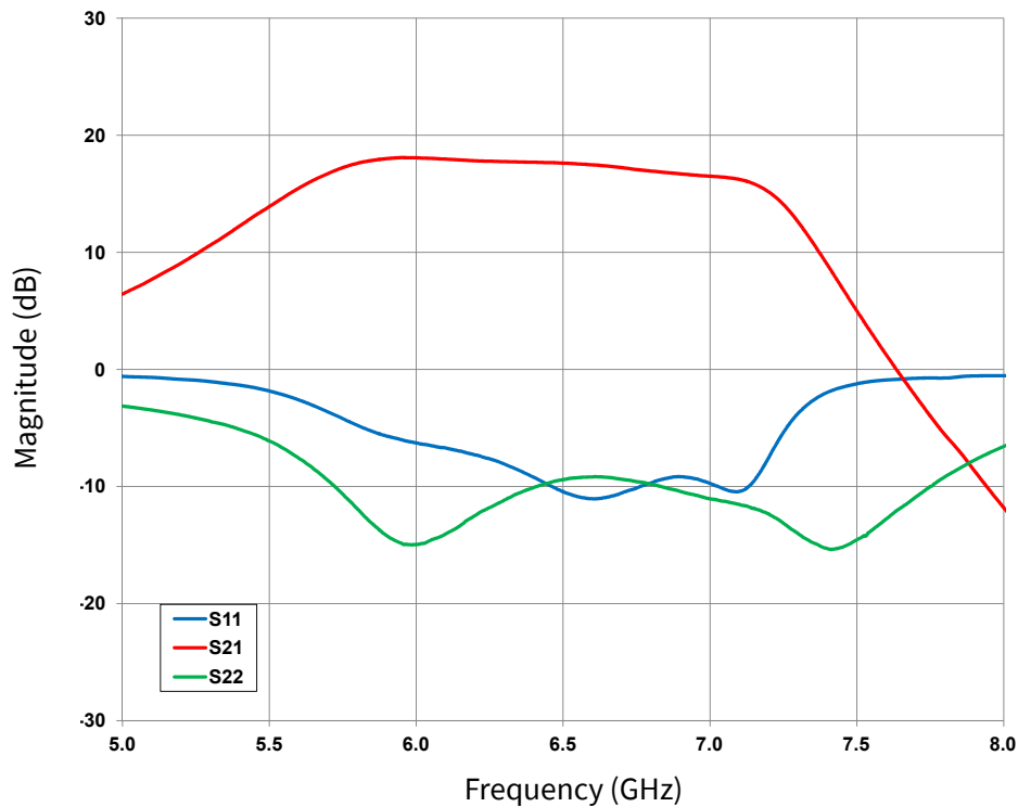
Figure 1. Typical Small Signal Response of CGHV1F006S-AMP1 Application Circuit
