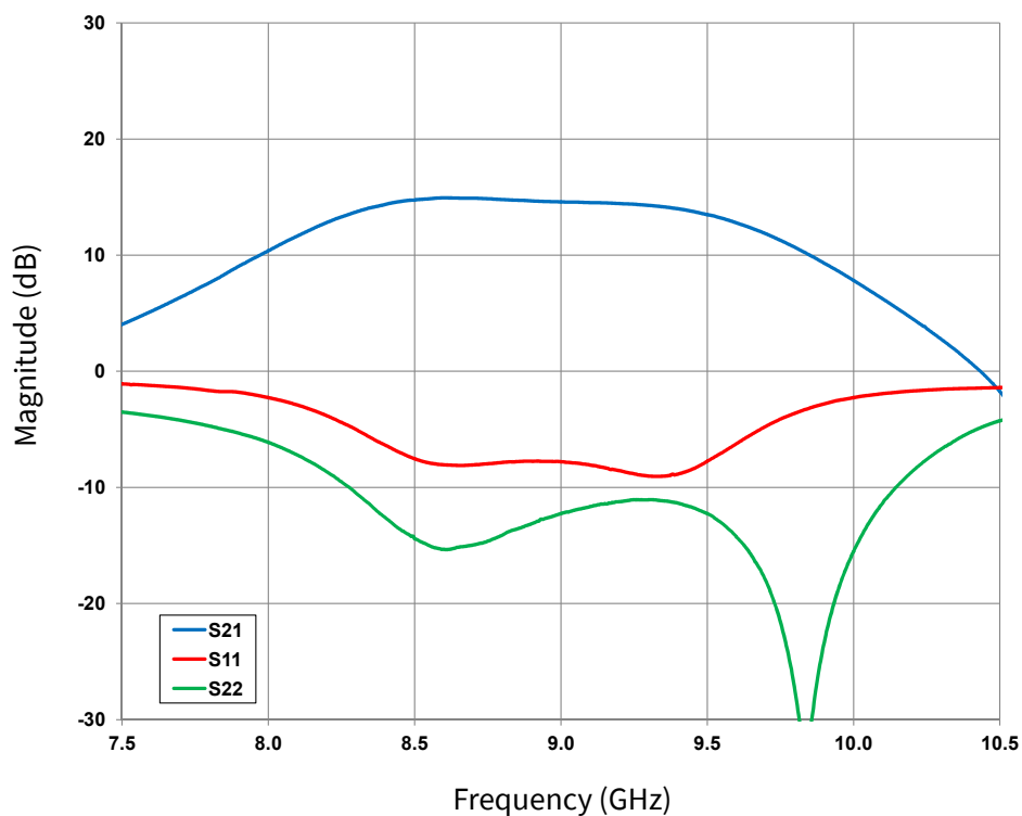
Figure 9. Typical Small Signal Response
