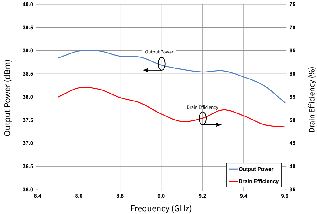
Figure 10. Typical Pulsed Power Response V_{DD} = 40\text{ V} , I_{DQ} = 60\text{ mA} , 100\text{ }\mu\text{s} , 10\% Duty, P_{IN} = 28\text{ dBm}
