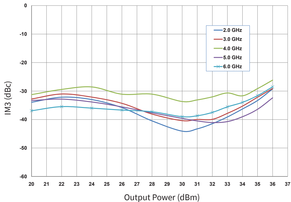
Third Order Intermodulation Distortion vs Average Output Power as a Function of Frequency of the CGH40006S in the CGH40006S-AMP1
