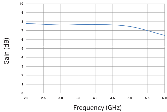
Output Power vs Frequency of the CGH40006S in the CGH40006S-AMP1 at P_{IN} = 32 \text{ dBm} , V_{DD} = 28 \text{ V}
