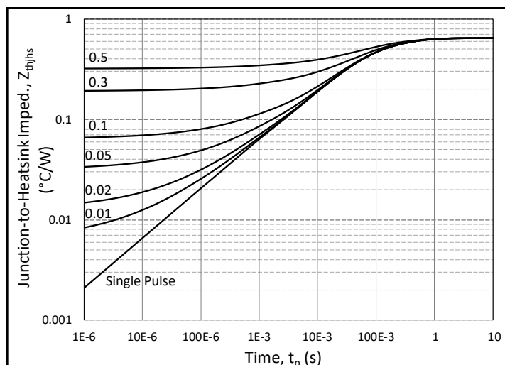
Figure 17. MOSFET Junction to Case Transient Thermal Impedance, Z_{thjcs} (°C/W)
