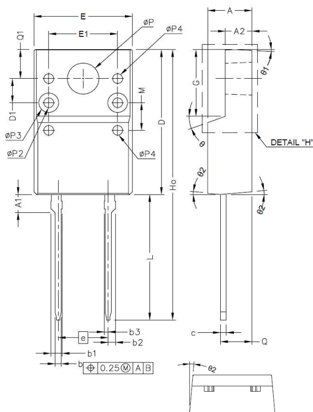
Package TO-220-F2
