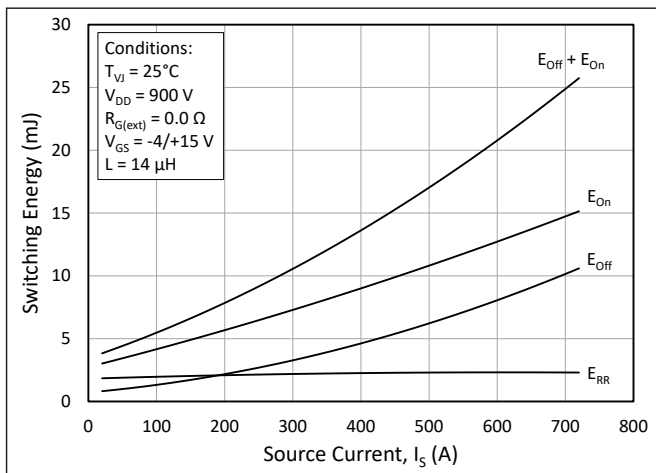
Figure 11. Switching Energy vs. Drain Current ( V_{DD} = 900\text{ V} )
